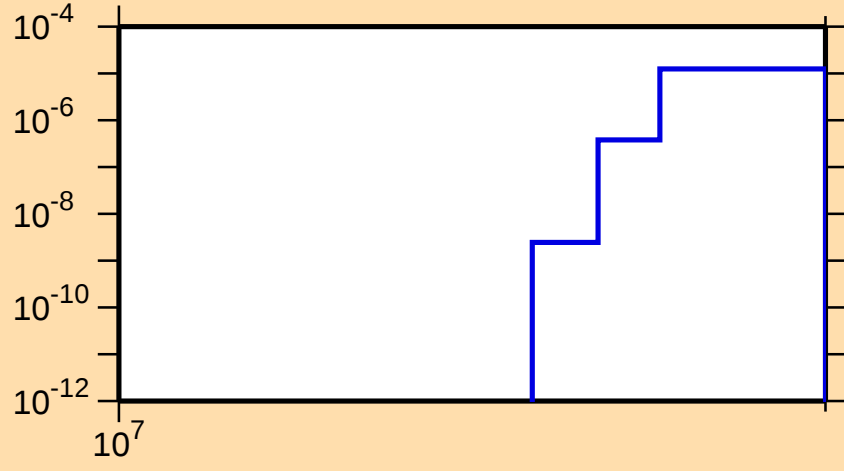
\sigma vs. E for ^{123}\text{Cd}(n,np)
