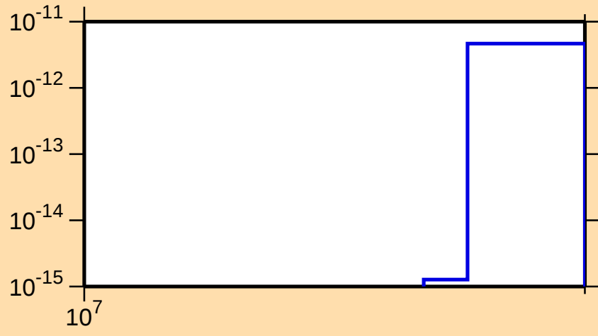
\sigma vs. E for ^{123}\text{Cd}(n,\text{nt})
