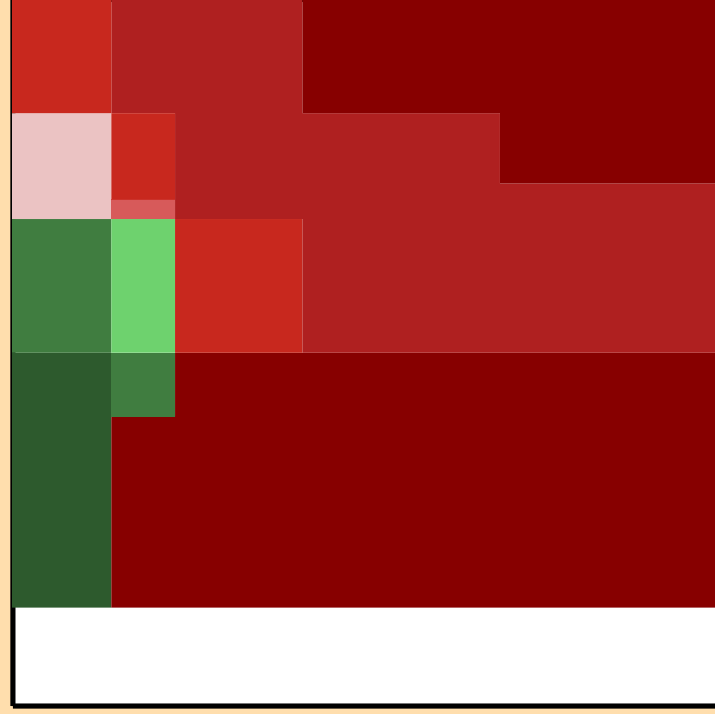
\Delta\sigma/\sigma vs. E for ^{123}\text{Cd}(n,\text{tot.})
