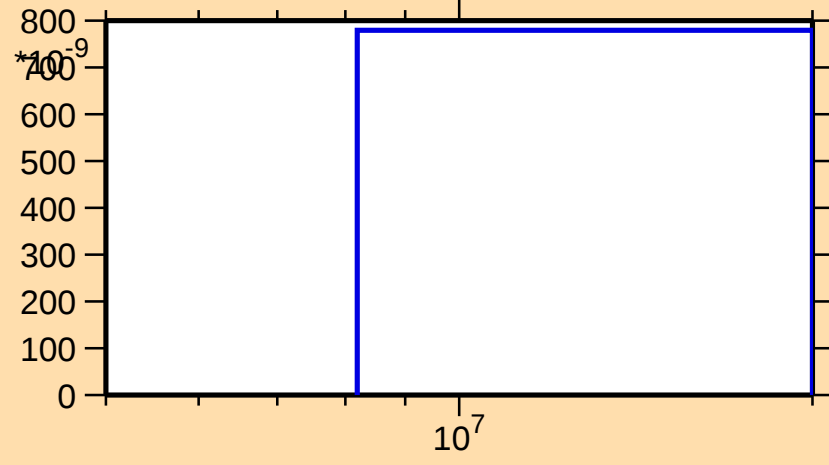
\sigma vs. E for ^{123}\text{Cd}(n,d)
