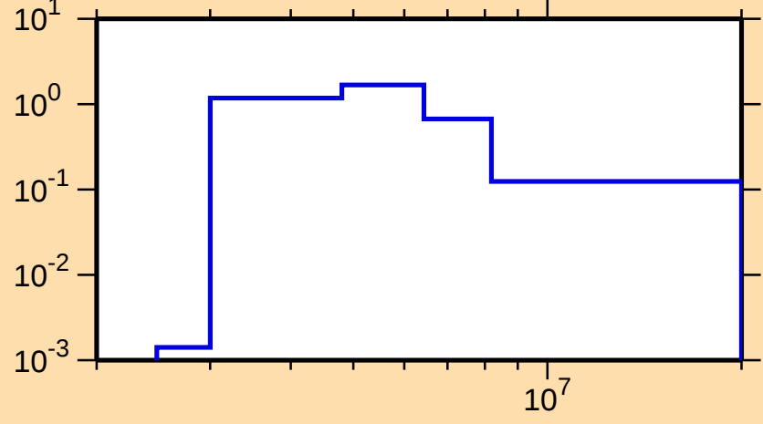
\sigma vs. E for ^{123}\text{Cd}(n,n\text{cont.})
