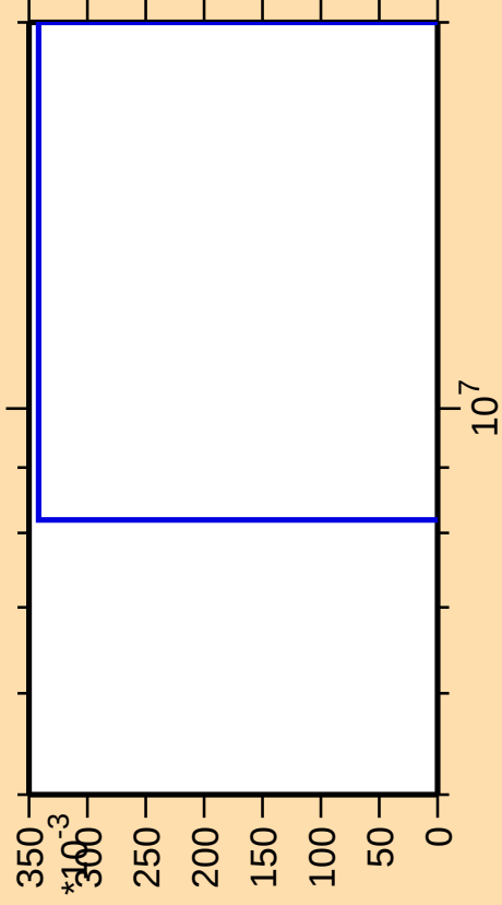
\Delta\sigma/\sigma vs. E for ^{123}\text{Cd}(n,\text{nt})
