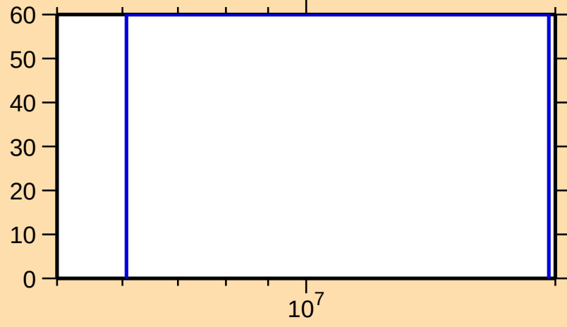
\Delta\sigma/\sigma vs. E for ^{123}\text{Cd}(n,p)
