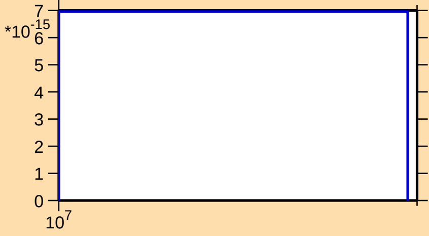
\sigma vs. E for ^{123}\text{Cd}(n,2n\alpha)
