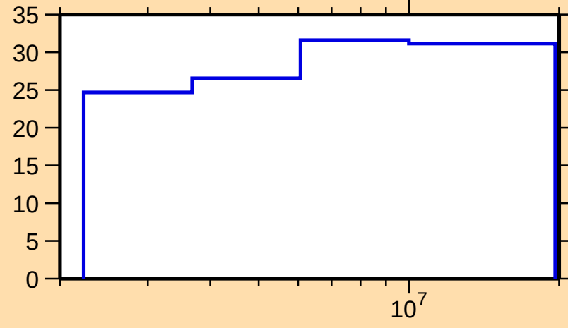
\Delta\sigma/\sigma vs. E for ^{123}\text{Cd}(\text{n},\text{nonel.})
