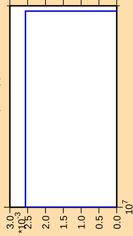
\Delta\sigma/\sigma vs. E for ^{123}\text{Cd}(n,2np)
