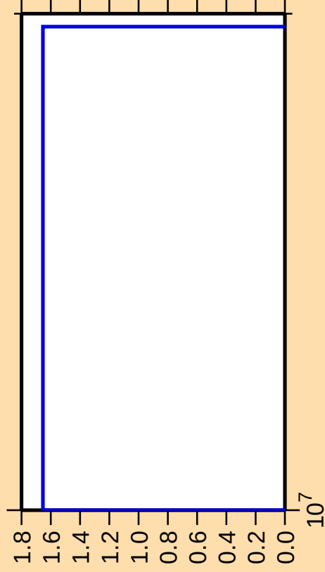
\Delta\sigma/\sigma vs. E for ^{123}\text{Cd}(n,\text{nt})
