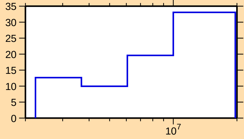
\Delta\sigma/\sigma vs. E for ^{123}\text{Cd}(\text{n},\text{tot.})
