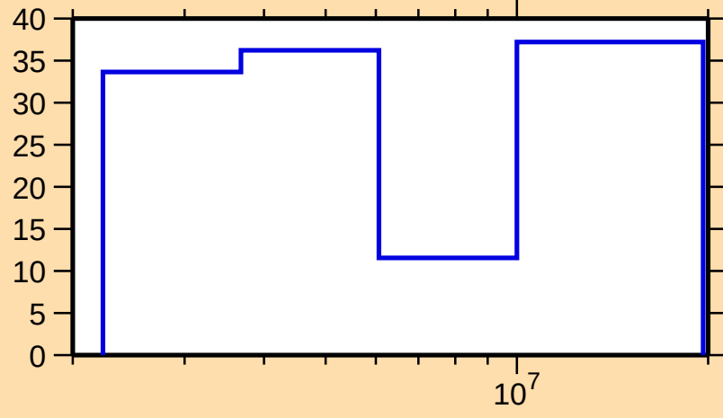
\Delta\sigma/\sigma vs. E for ^{123}\text{Cd}(\text{n},\text{el.})
