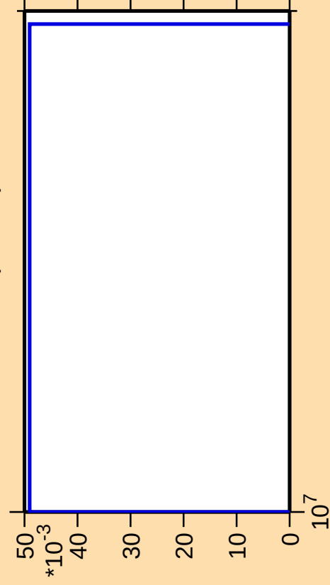
\Delta\sigma/\sigma vs. E for ^{123}\text{Cd}(n,2n\alpha)
