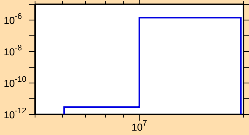
\sigma vs. E for ^{123}\text{Cd}(n,\alpha)
