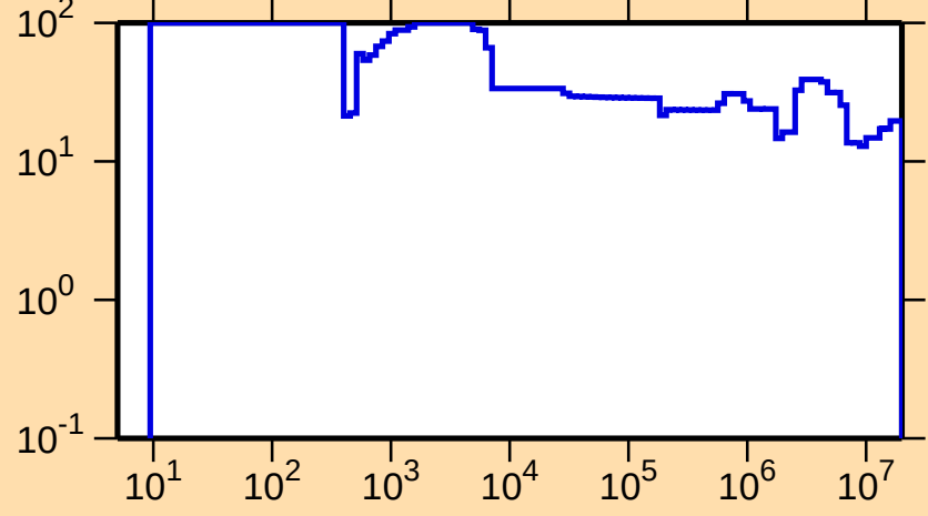
\Delta\sigma/\sigma vs. E for ^{124}\text{Cd}(n,\text{tot.})
