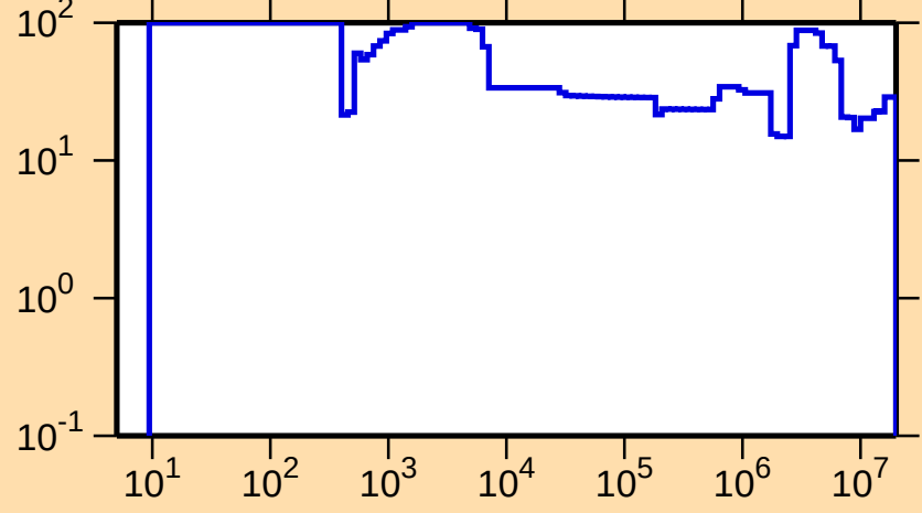
\Delta\sigma/\sigma vs. E for ^{124}\text{Cd}(n,\text{el.})
