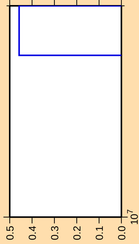
\Delta\sigma/\sigma vs. E for ^{124}\text{Cd}(n,\text{nt})
