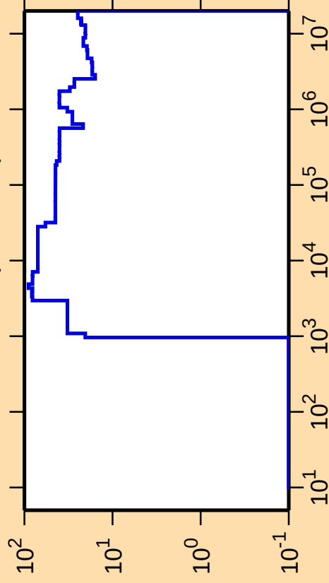
\Delta\sigma/\sigma vs. E for ^{124}\text{Cd}(n,\text{nonel.})
