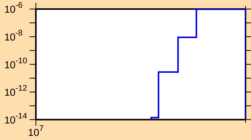
\sigma vs. E for ^{124}\text{Cd}(n,t)
