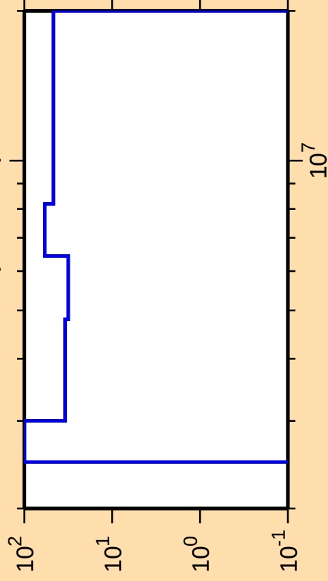
\Delta\sigma/\sigma vs. E for ^{124}\text{Cd}(\text{n},\text{ncont.})
