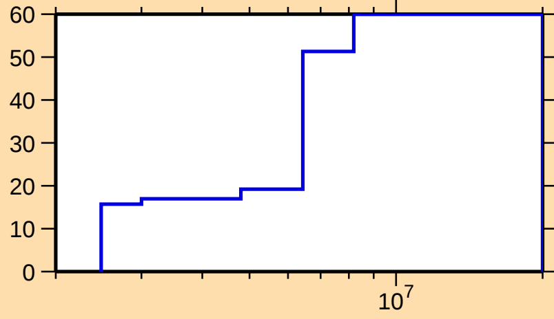
\Delta\sigma/\sigma vs. E for ^{124}\text{Cd}(\text{n},\text{inel.})
