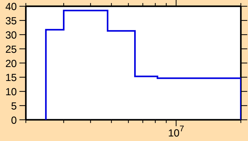
\Delta\sigma/\sigma vs. E for ^{124}\text{Cd}(\text{n},\text{tot.})
