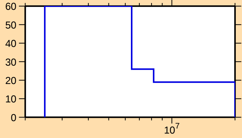
\Delta\sigma/\sigma vs. E for ^{124}\text{Cd}(\text{n},\text{el.})
