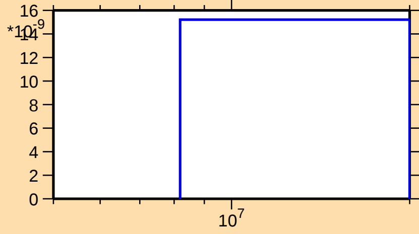
\sigma vs. E for ^{124}\text{Cd}(n,np)
