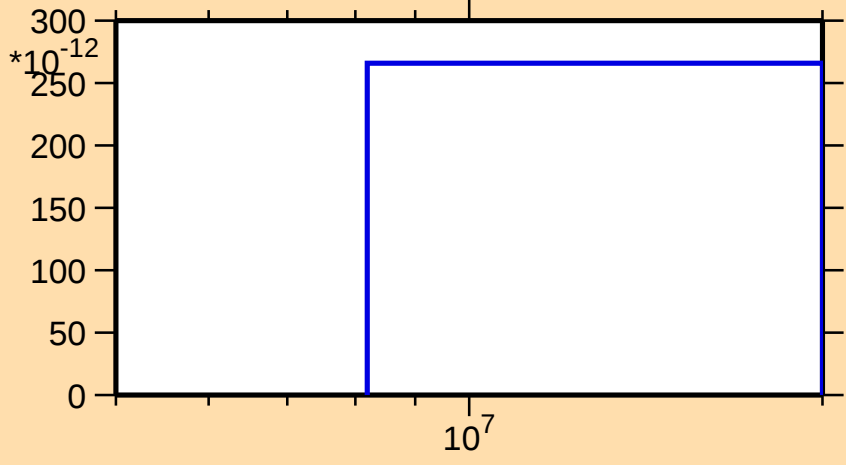
\sigma vs. E for ^{124}\text{Cd}(n,\alpha)
