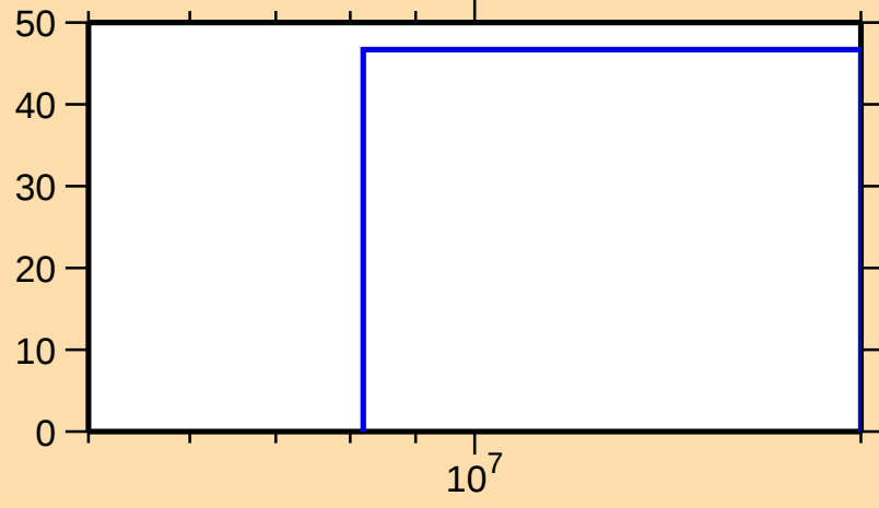
\Delta\sigma/\sigma vs. E for ^{124}\text{Cd}(n,\text{ncont.})
