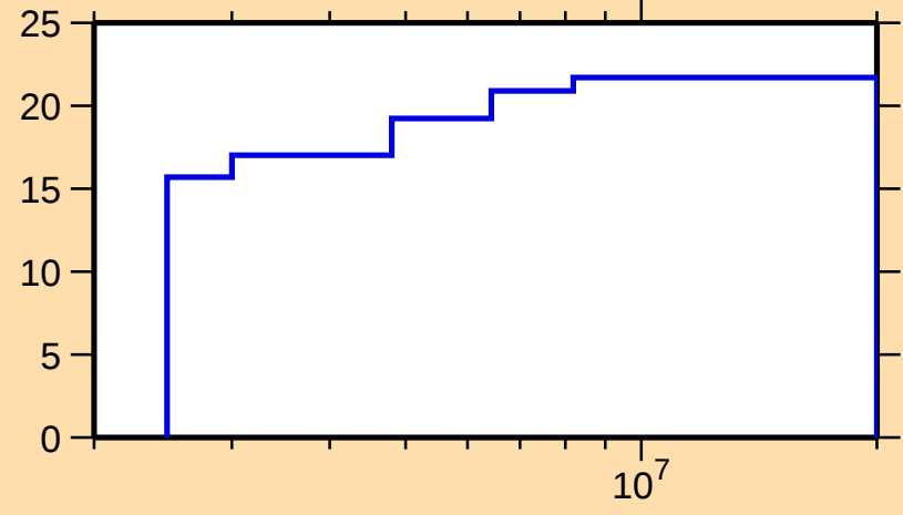
\Delta\sigma/\sigma vs. E for ^{124}\text{Cd}(\text{n},\text{nonel.})
