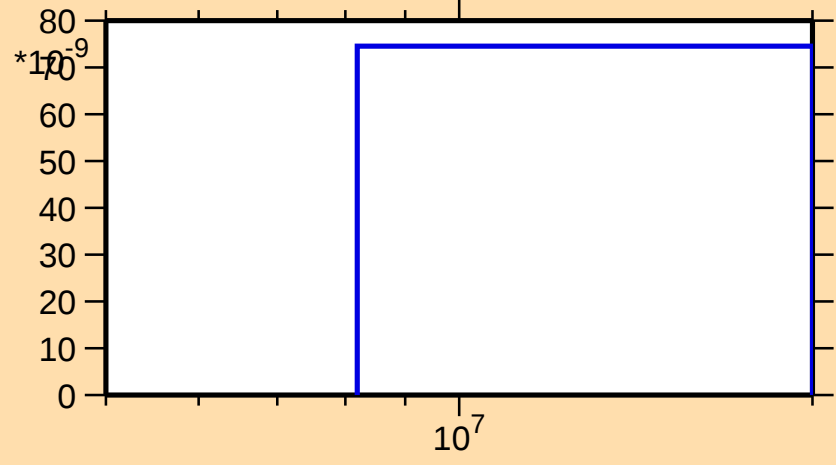
\sigma vs. E for ^{124}\text{Cd}(n,d)
