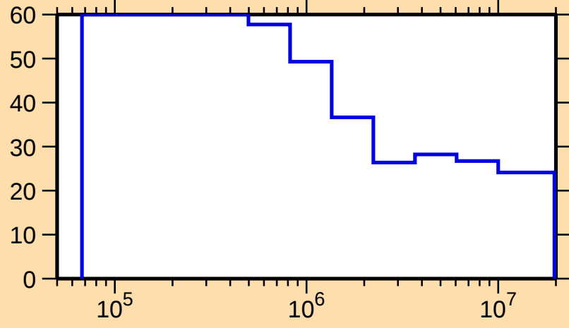
\Delta\sigma/\sigma vs. E for ^{283}_{11}
