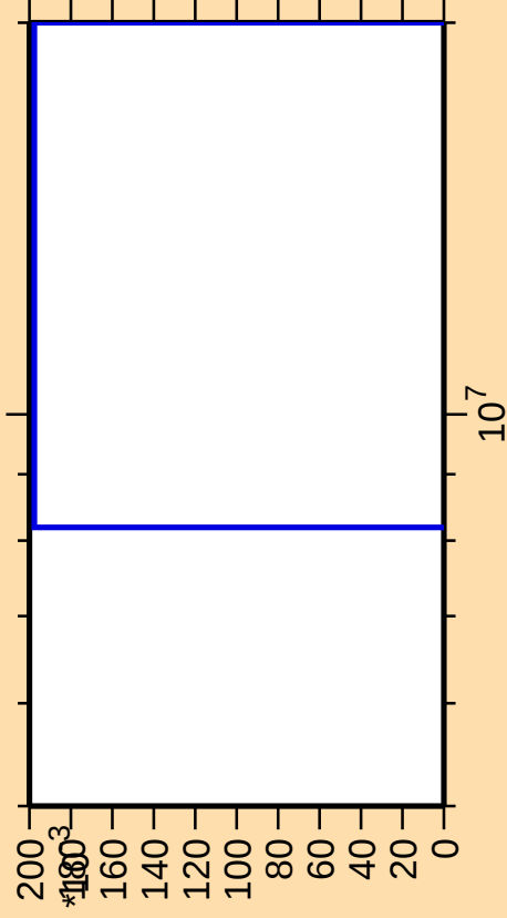
\Delta\sigma/\sigma vs. E for ^{283}\text{He3}
