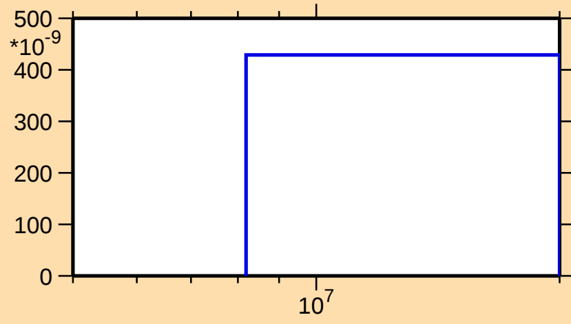
\sigma vs. E for ^{283}
