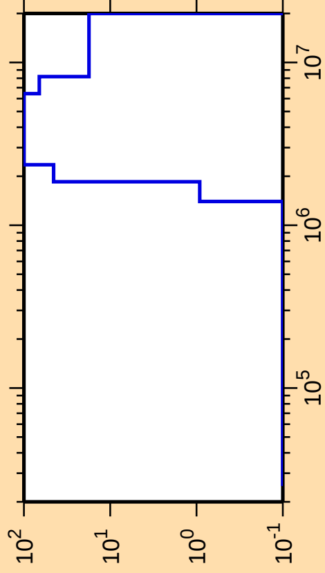
\Delta\sigma/\sigma vs. E for ^{283}_{11}
