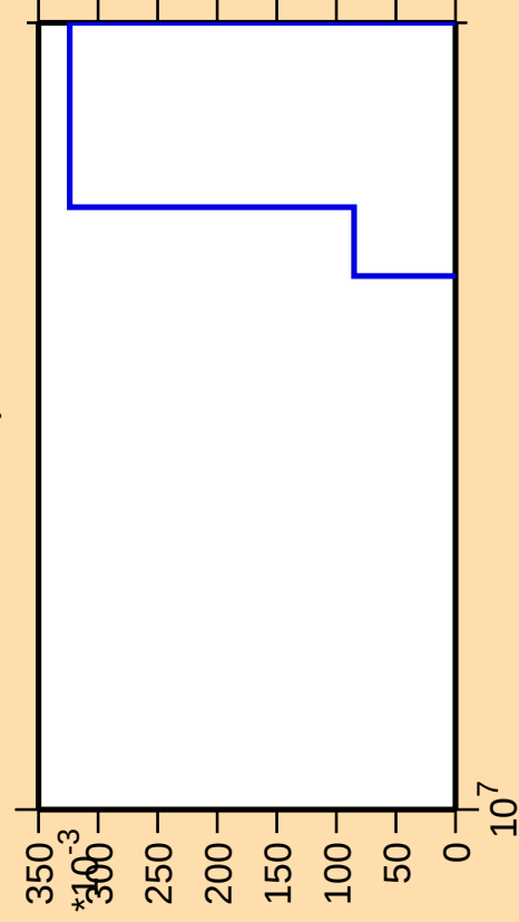
\Delta\sigma/\sigma vs. E for ^{285}\text{He3} )
