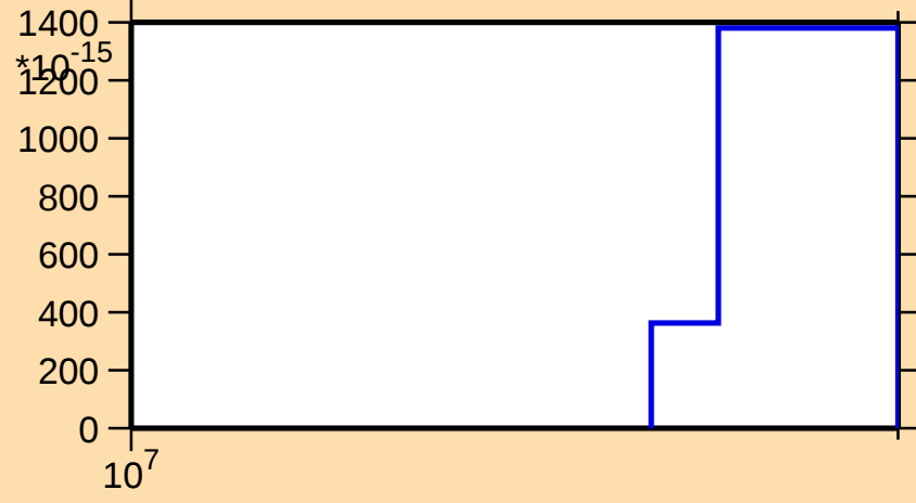
\sigma vs. E for ^{285}\text{He3} )
