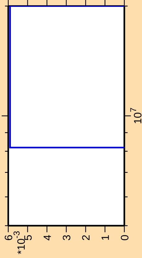
\Delta\sigma/\sigma vs. E for ^{285}\text{He3}
