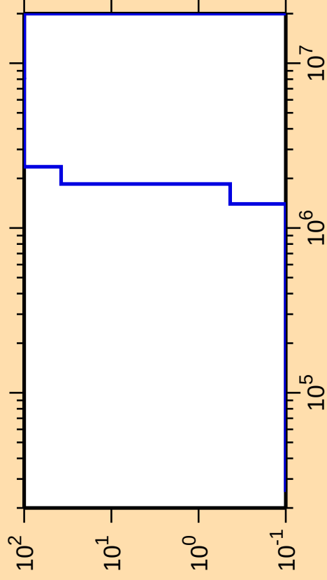
\Delta\sigma/\sigma vs. E for ^{285}_{111}
