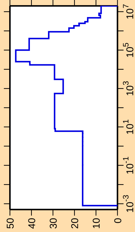
\Delta\sigma/\sigma vs. E for ^{285}
