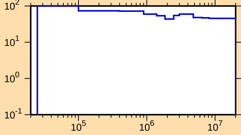
\Delta\sigma/\sigma vs. E for ^{285}_{111}
