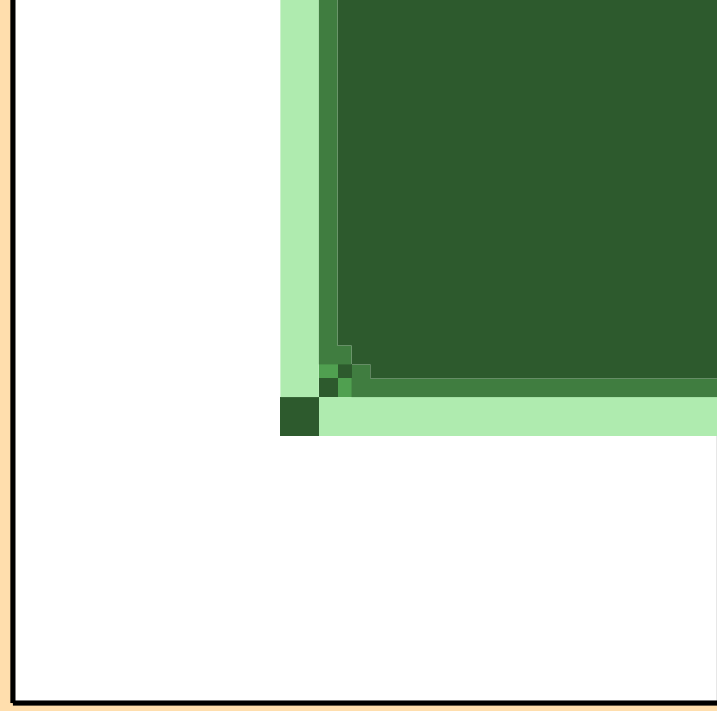
\sigma vs. E for ^{54}\text{Co}(n,2n)
