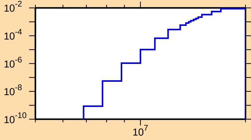
\sigma vs. E for ^{54}\text{Co}(n,\text{He3})
