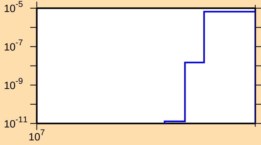
\sigma vs. E for ^{54}\text{Co}(n,2np)
