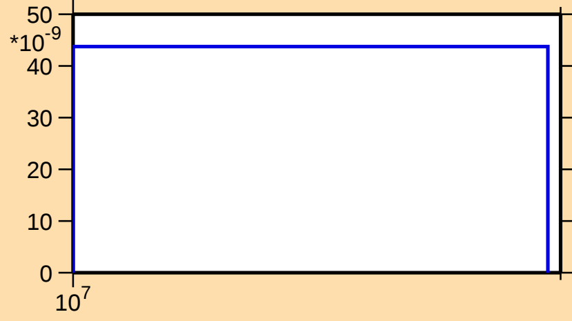
\sigma vs. E for ^{54}\text{Co}(n,\text{pt})
