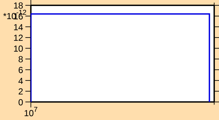
\sigma vs. E for ^{54}\text{Co}(\text{mt } 34)
