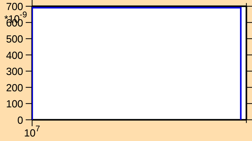
\sigma vs. E for ^{54}\text{Co}(n,\text{nd})
