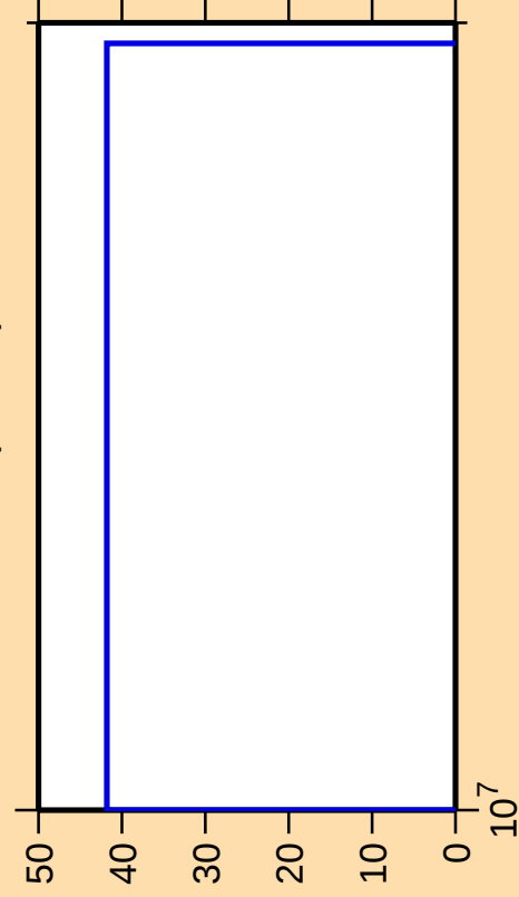
\Delta\sigma/\sigma vs. E for ^{54}\text{Co}(\text{mt } 34)
