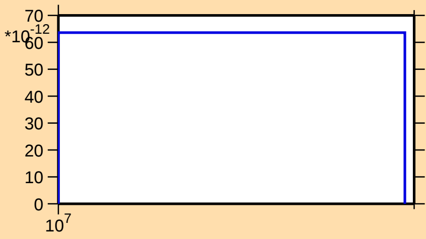
\sigma vs. E for ^{54}\text{Co}(\text{mt117})
