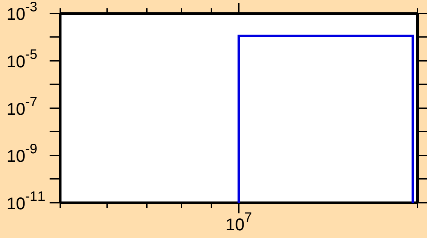
\sigma vs. E for ^{54}\text{Co}(n,n\alpha)
