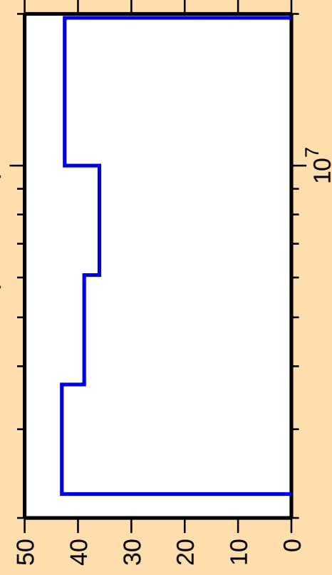
\Delta\sigma/\sigma vs. E for ^{54}\text{Co}(n,n\text{cont.})
