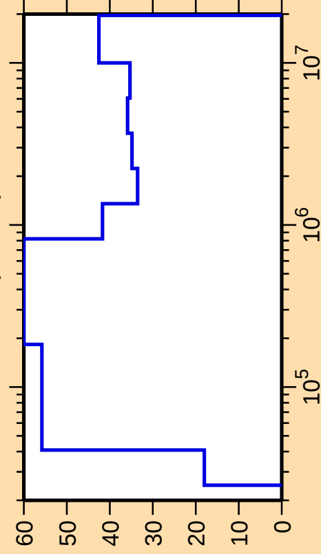
\Delta\sigma/\sigma vs. E for ^{54}\text{Co}(n,\text{inel.})
