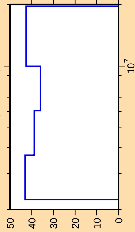
\Delta\sigma/\sigma vs. E for ^{54}\text{Co}(n,\text{ncont.})
