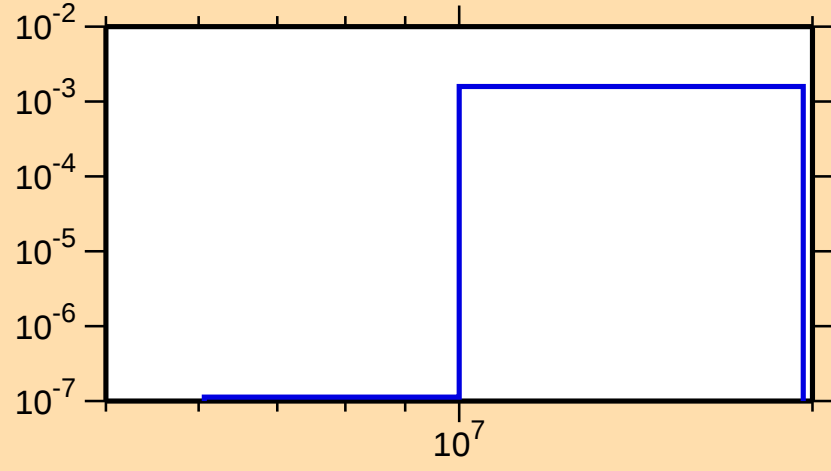
\sigma vs. E for ^{54}\text{Co}(n,\text{He3})
