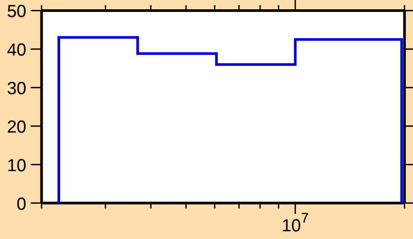
\Delta\sigma/\sigma vs. E for ^{54}\text{Co}(n,n\text{cont.})
