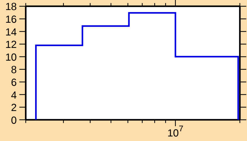
\Delta\sigma/\sigma vs. E for ^{54}\text{Co}(n,\text{el.})
