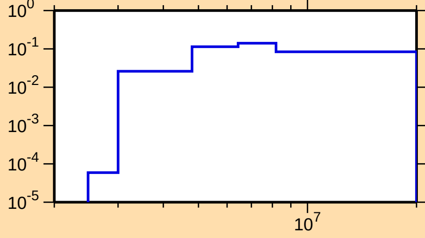
\sigma vs. E for ^{54}\text{Co}(n,n\text{cont.})
