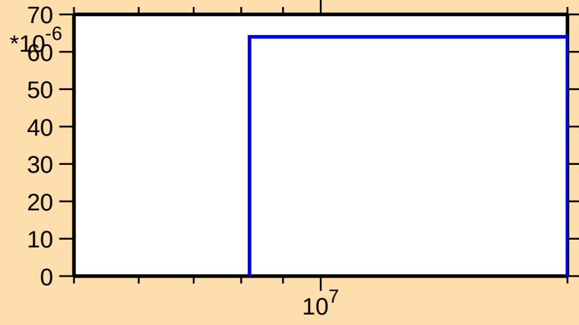
\sigma vs. E for ^{54}\text{Co}(n,2n)
