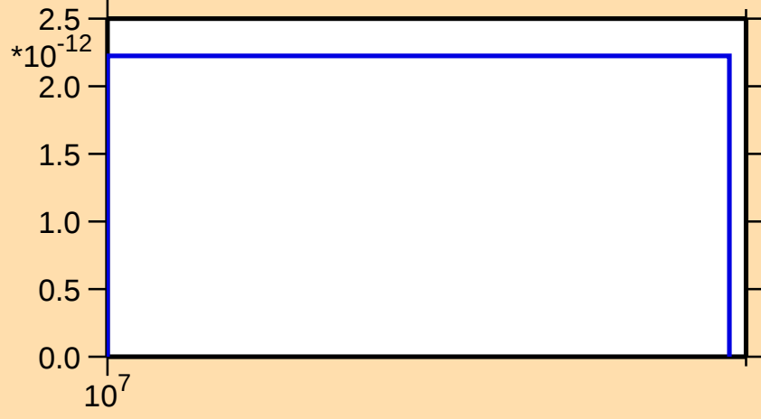
\sigma vs. E for ^{55}\text{Co}(\text{mt } 45)
