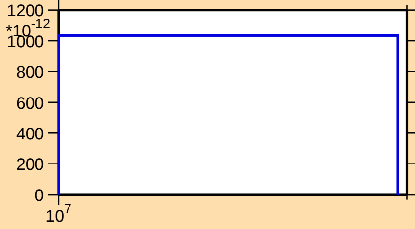
\sigma vs. E for ^{55}\text{Co}(n,\text{nd})
