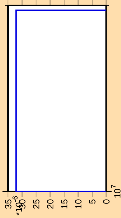
\Delta\sigma/\sigma vs. E for ^{55}\text{Co}(\text{mt } 34)
