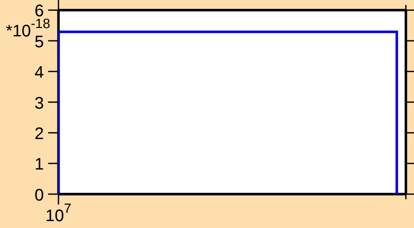
\sigma vs. E for ^{55}\text{Co}(\text{mt } 34)
