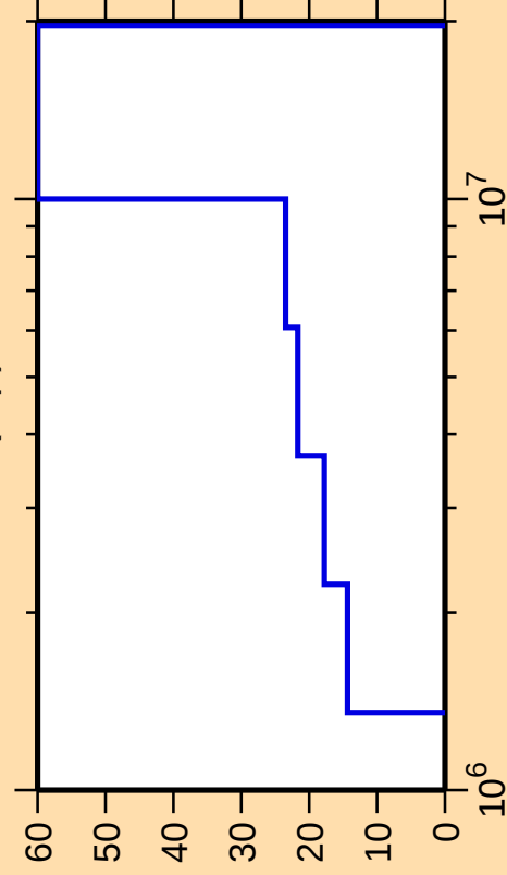
\Delta\sigma/\sigma vs. E for ^{55}\text{Co}(n,p)
