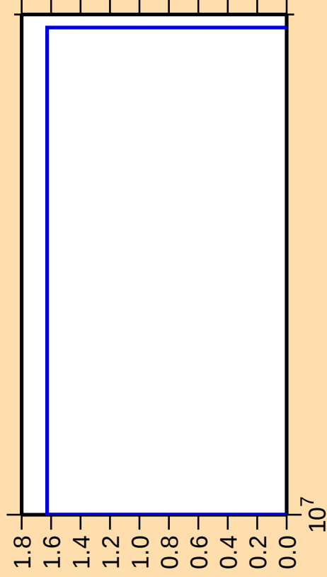
\Delta\sigma/\sigma vs. E for ^{55}\text{Co}(\text{mt } 45)
