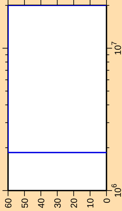
\Delta\sigma/\sigma vs. E for ^{55}\text{Co}(n,\gamma)
