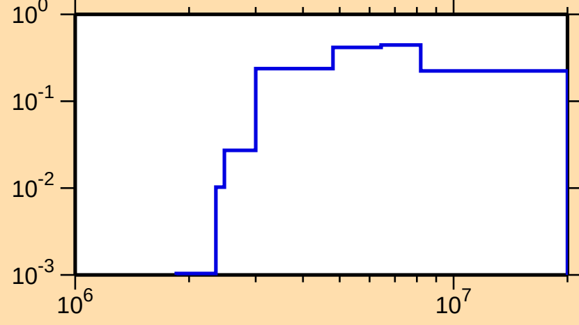
\sigma vs. E for ^{55}\text{Co}(n,\text{inel.})
