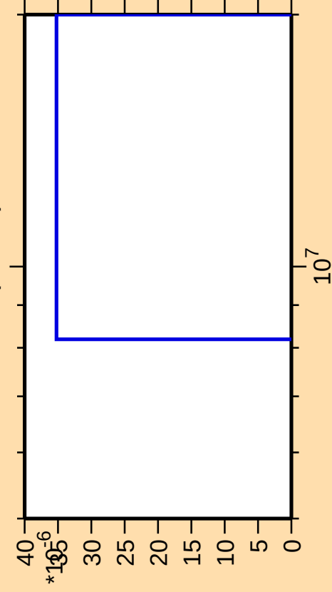
\Delta\sigma/\sigma vs. E for ^{55}\text{Co}(\text{mt } 34)
