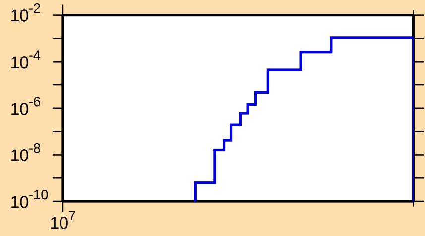
\sigma vs. E for ^{48}\text{Cr}(n,\text{pd})
