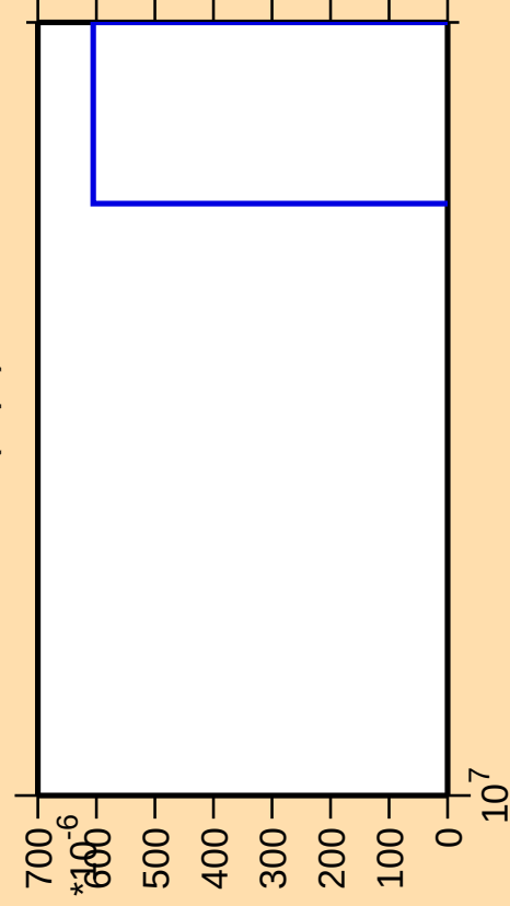
\Delta\sigma/\sigma vs. E for ^{48}\text{Cr}(n,\text{pt})
