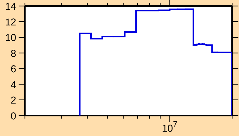
\Delta\sigma/\sigma vs. E for ^{48}\text{Cr}(n,\text{el.})
