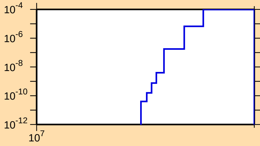
\sigma vs. E for ^{48}\text{Cr}(n,t)
