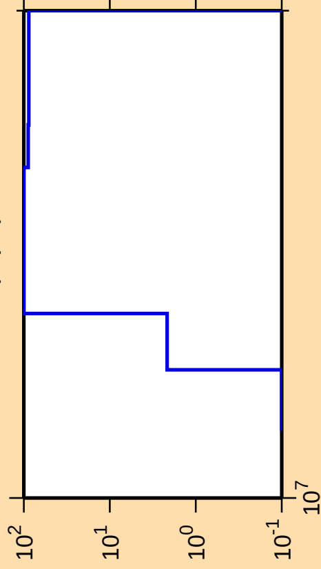
\Delta\sigma/\sigma vs. E for ^{48}\text{Cr}(n,\text{pd})
