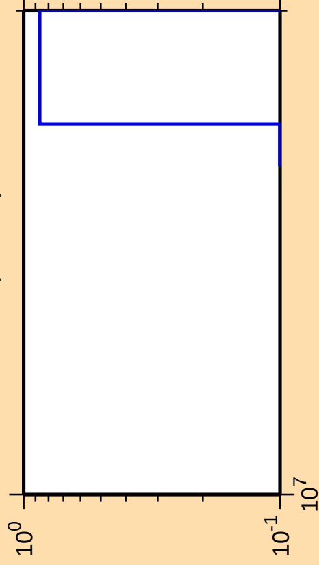
\Delta\sigma/\sigma vs. E for ^{48}\text{Cr}(\text{mt117})
