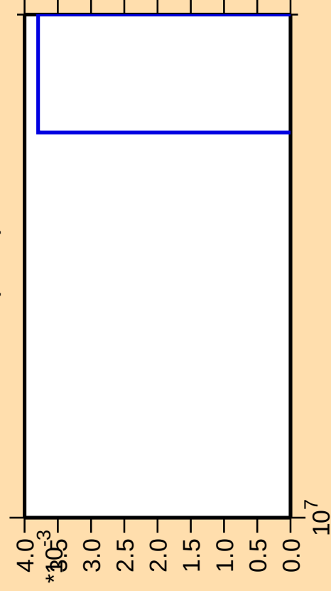
\Delta\sigma/\sigma vs. E for ^{48}\text{Cr}(n,\text{nd})
