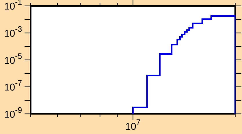
\sigma vs. E for ^{48}\text{Cr}(n,n\alpha)
