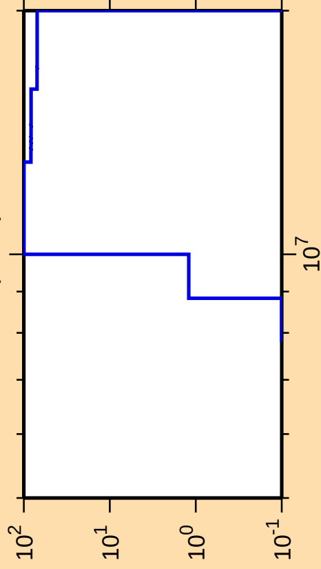
\Delta\sigma/\sigma vs. E for ^{48}\text{Cr}(n,n\alpha)
