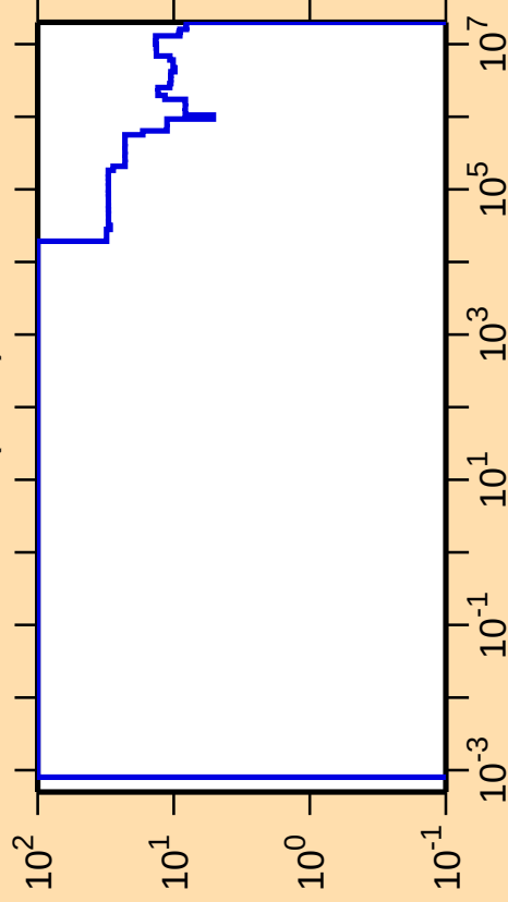
\Delta\sigma/\sigma vs. E for ^{48}\text{Cr}(n,\text{el.})
