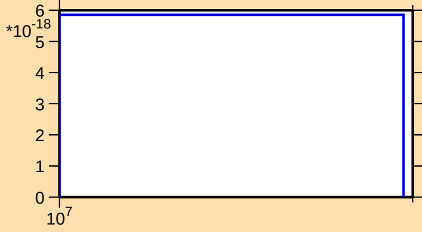
\sigma vs. E for ^{48}\text{Cr}(n,\text{nd})
