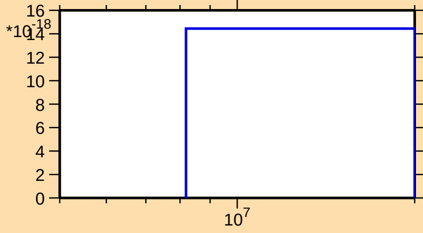
\sigma vs. E for ^{48}\text{Cr}(n,nd)
