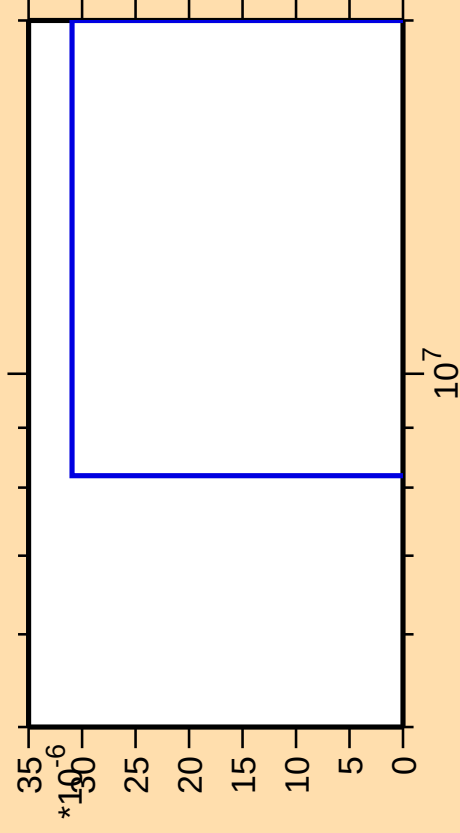
\Delta\sigma/\sigma vs. E for ^{48}\text{Cr}(n,nd)
