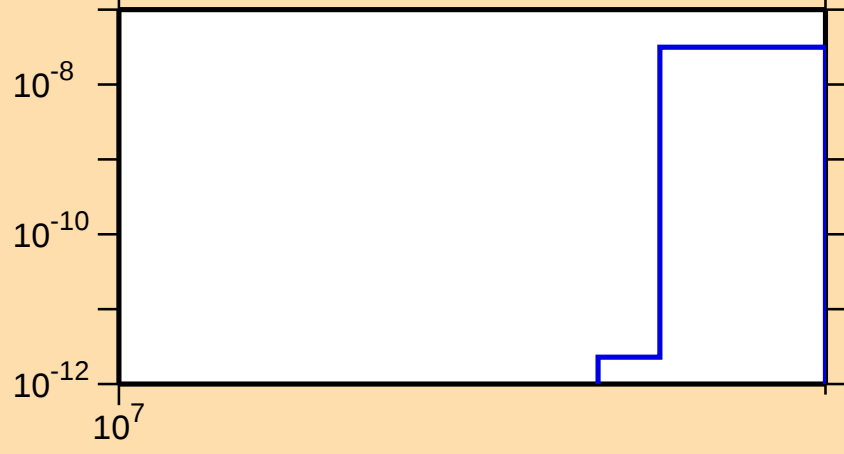
\sigma vs. E for ^{57}\text{Cr}(n,2n\alpha)
