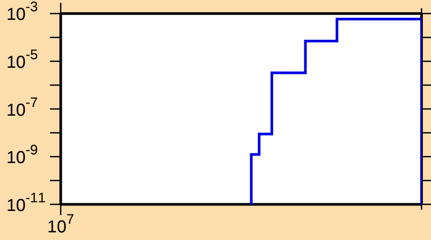
\sigma vs. E for ^{57}\text{Cr}(n,np)
