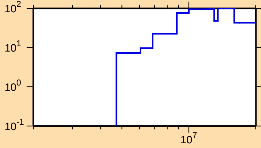
\Delta\sigma/\sigma vs. E for ^{57}\text{Cr}(n,n_1)
