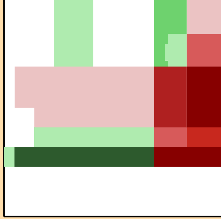
\Delta\sigma/\sigma vs. E for ^{57}\text{Cr}(n,ncont.)
