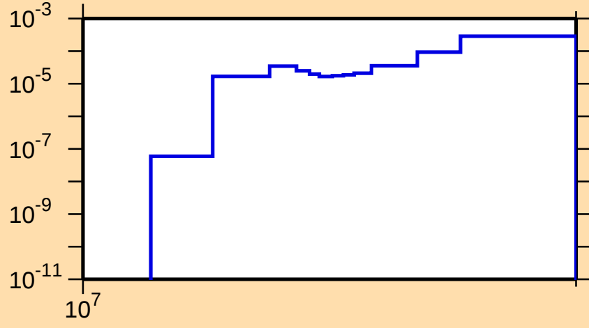
\sigma vs. E for ^{57}\text{Cr}(n,t)
