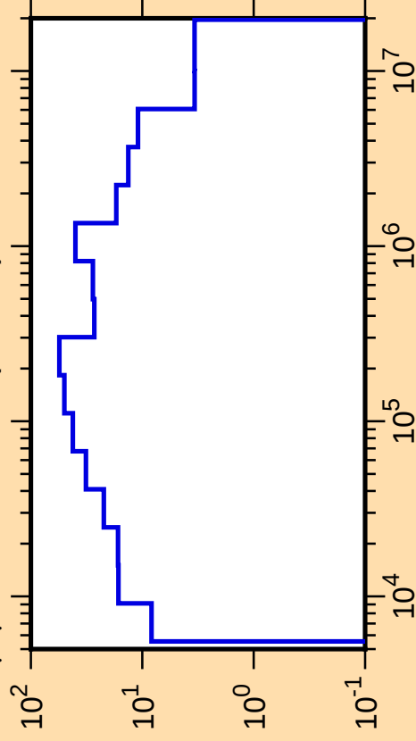
\Delta\mu/\mu vs. E for ^{57}\text{Cr}(\text{mt251})
