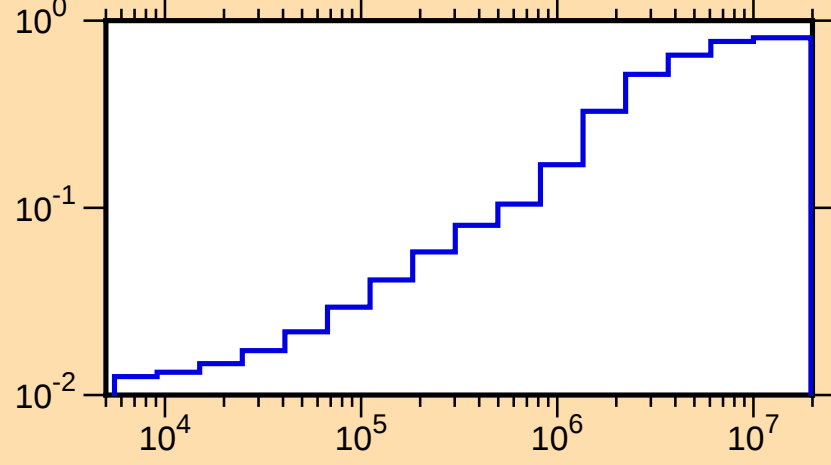
\mu vs. E for ^{57}\text{Cr}(\text{mt251})
