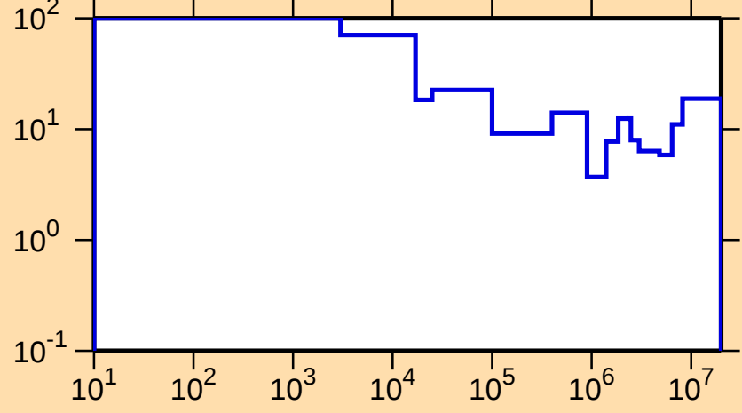
\Delta\sigma/\sigma vs. E for ^{57}\text{Cr}(n,\text{el.})
