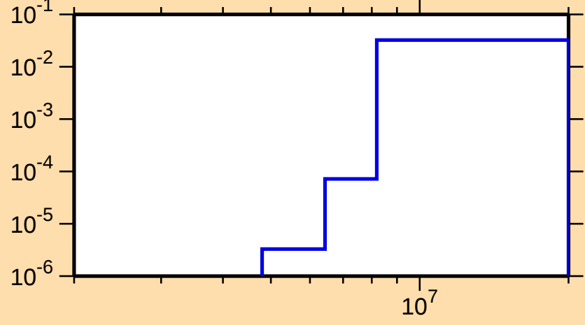
\sigma vs. E for ^{57}\text{Cr}(n,n\text{cont.})
