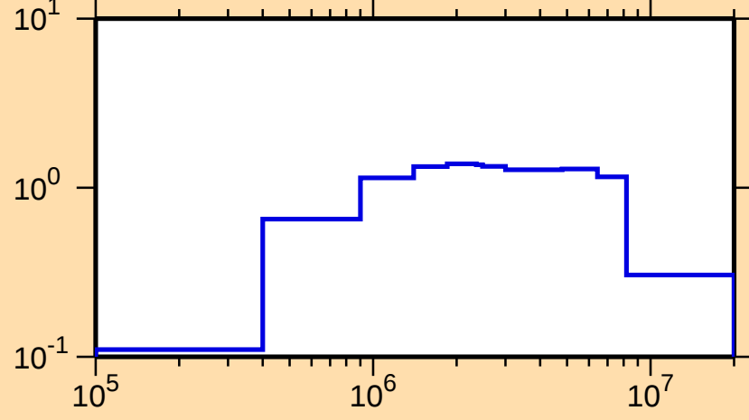
\sigma vs. E for ^{57}\text{Cr}(n,\text{inel.})
