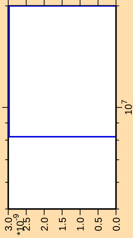
\Delta\sigma/\sigma vs. E for ^{57}\text{Cr}(n,\text{He3})
