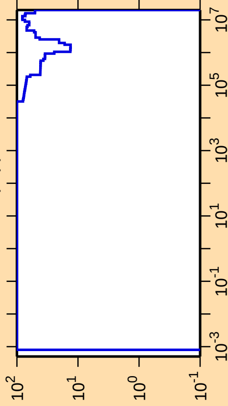
\Delta\sigma/\sigma vs. E for ^{117}\text{Cs}(n,p)
