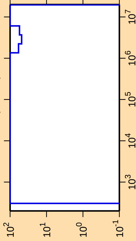
\Delta\sigma/\sigma vs. E for ^{117}\text{Cs}(n,\text{inel.})
