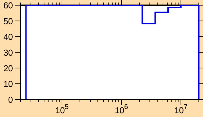
\Delta\sigma/\sigma vs. E for ^{117}\text{Cs}(n,n_1)
