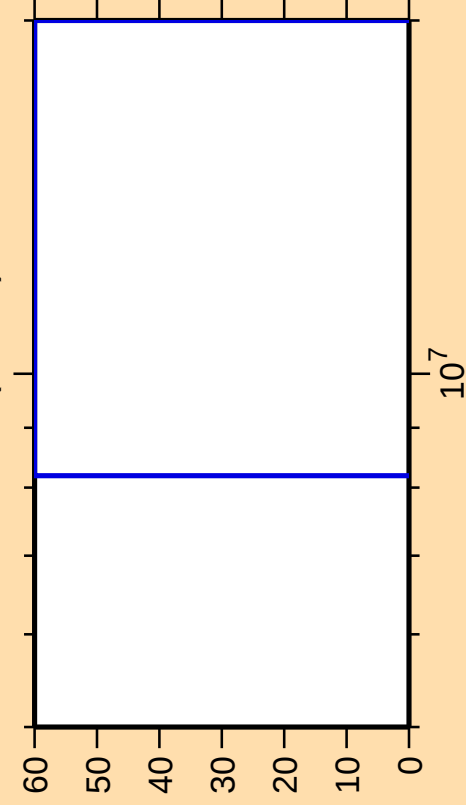
\Delta\sigma/\sigma vs. E for ^{117}\text{Cs}(\text{mt } 34)
