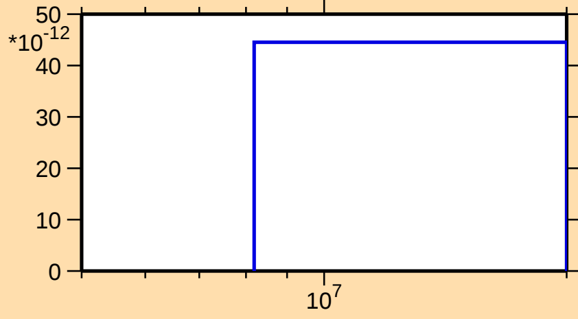
\sigma vs. E for ^{117}\text{Cs}(\text{mt } 34)
