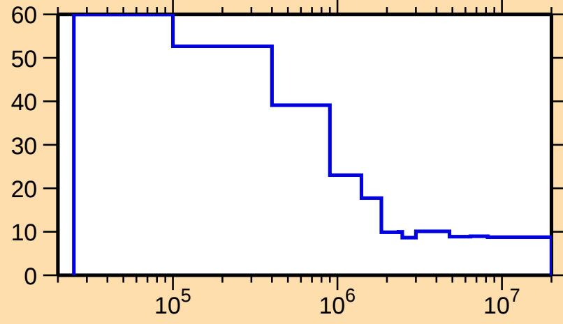
\Delta\sigma/\sigma vs. E for ^{117}\text{Cs}(n,n\text{onel.})
