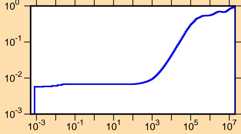
\mu vs. E for ^{119}\text{Cs}(\text{mt251})
