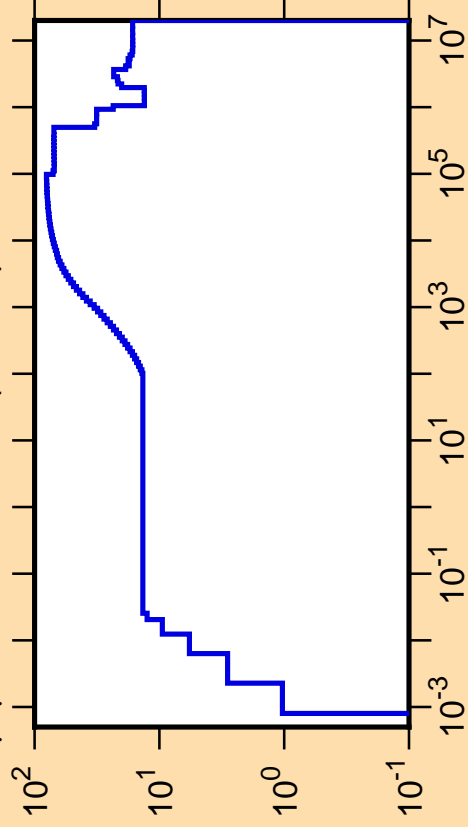
\Delta\mu/\mu vs. E for ^{119}\text{Cs}(\text{mt251})
