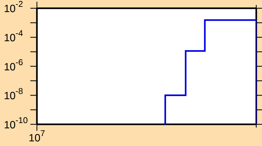
\sigma vs. E for ^{123}\text{Cs}(n,2np)
