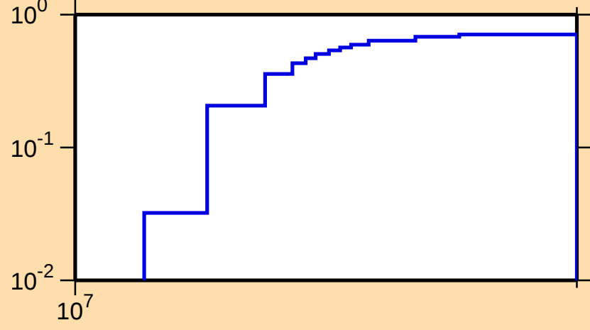
\sigma vs. E for ^{123}\text{Cs}(n,2n)
