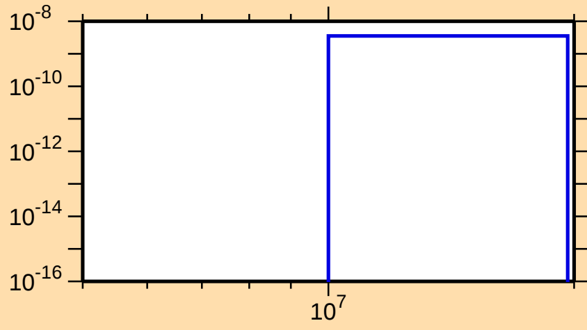
\sigma vs. E for ^{123}\text{Cs}(\text{mt117})
