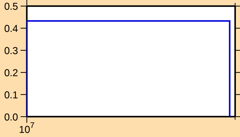
\sigma vs. E for ^{123}\text{Cs}(n,2n)
