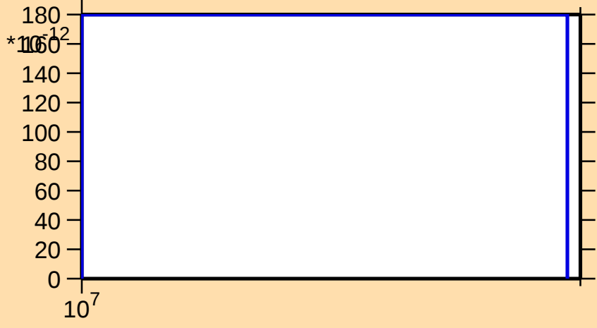
\sigma vs. E for ^{123}\text{Cs}(n,nt)
