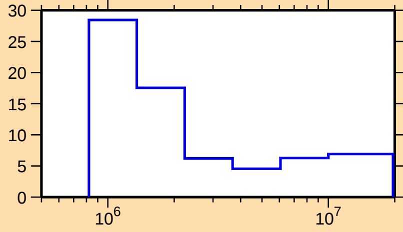
\Delta\sigma/\sigma vs. E for ^{123}\text{Cs}(n,n\text{onel.})
