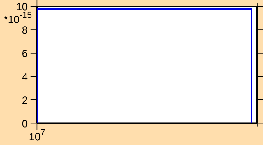
\sigma vs. E for ^{123}\text{Cs}(\text{mt } 34)
