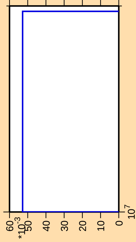
\Delta\sigma/\sigma vs. E for ^{123}\text{Cs}(\text{mt } 34)
