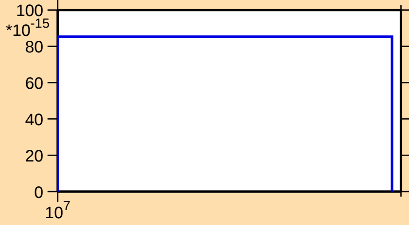
\sigma vs. E for ^{123}\text{Cs}(n,\text{pt})
