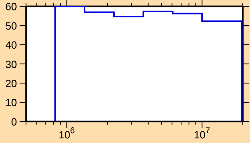
\Delta\sigma/\sigma vs. E for ^{123}\text{Cs}(n,n_1)
