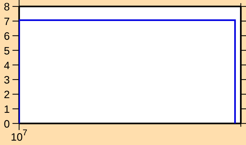
\Delta\sigma/\sigma vs. E for ^{123}\text{Cs}(n,\text{nonel.})
