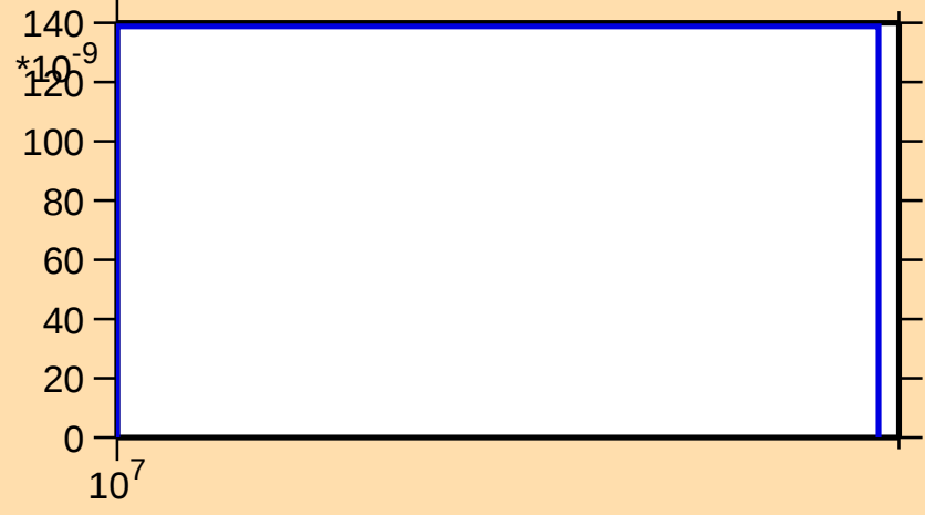
\sigma vs. E for ^{123}\text{Cs}(n,\text{nd})
