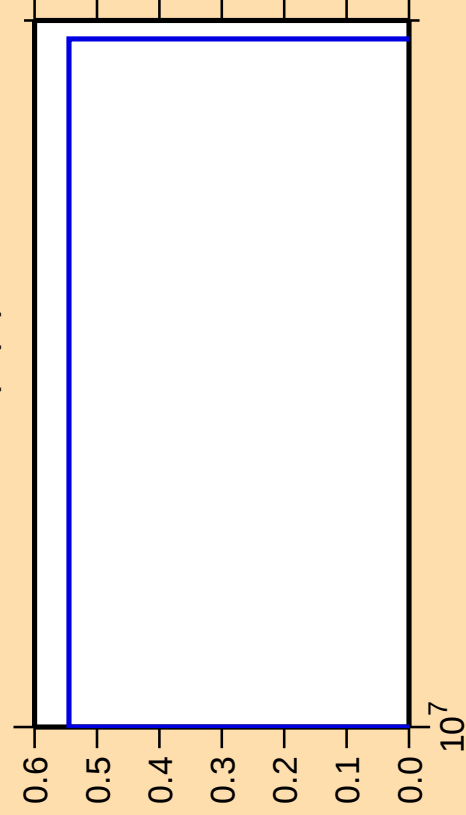
\Delta\sigma/\sigma vs. E for ^{123}\text{Cs}(n,\text{pt})
