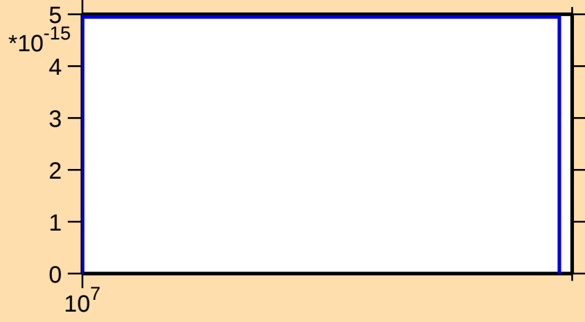
\sigma vs. E for ^{123}\text{Cs} (mt 34)
