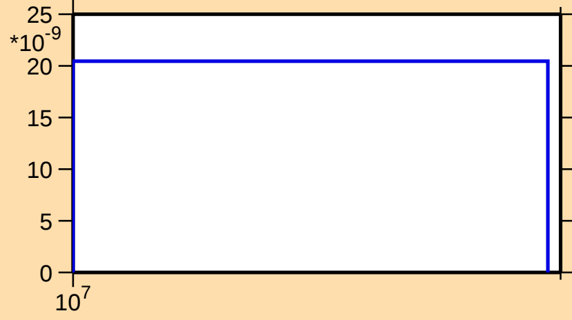
\sigma vs. E for ^{123}\text{Cs}(n,\text{pd})
