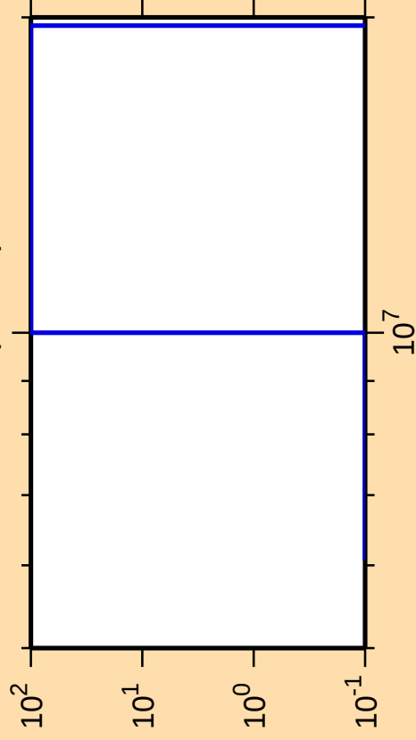
\Delta\sigma/\sigma vs. E for ^{123}\text{Cs}(\text{mt } 45)
