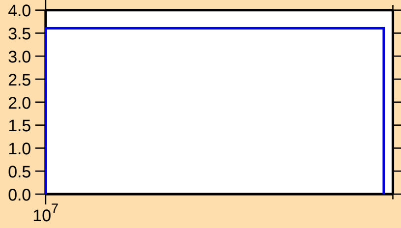
\Delta\sigma/\sigma vs. E for ^{123}\text{Cs}(n,\text{el.})
