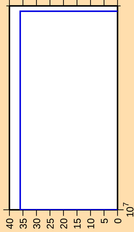
\Delta\sigma/\sigma vs. E for ^{123}\text{Cs}(n,2n)
