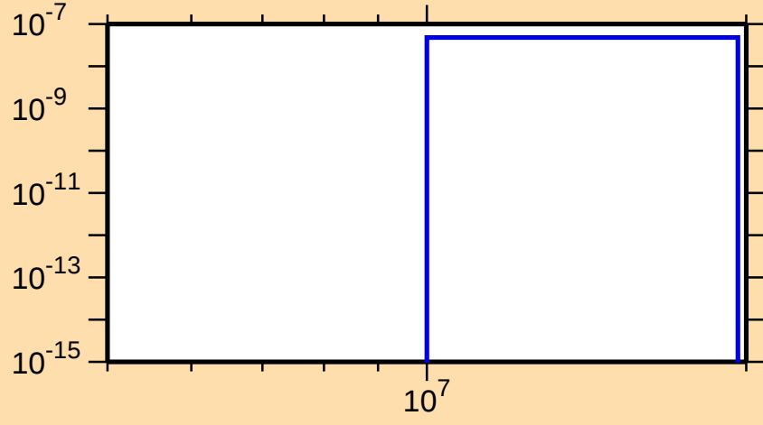
\sigma vs. E for ^{123}\text{Cs}(\text{mt } 45)
