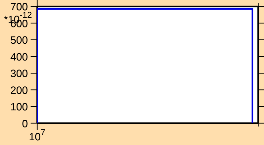
\sigma vs. E for ^{123}\text{Cs}(\text{mt117})
