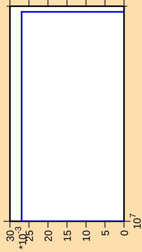
\Delta\sigma/\sigma vs. E for ^{123}\text{Cs} (mt 34)
