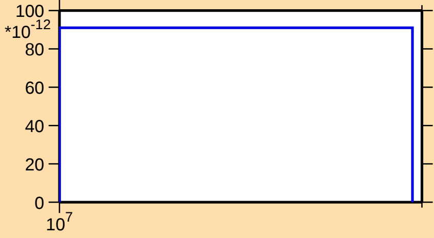
\sigma vs. E for ^{123}\text{Cs}(n,\text{nt})
