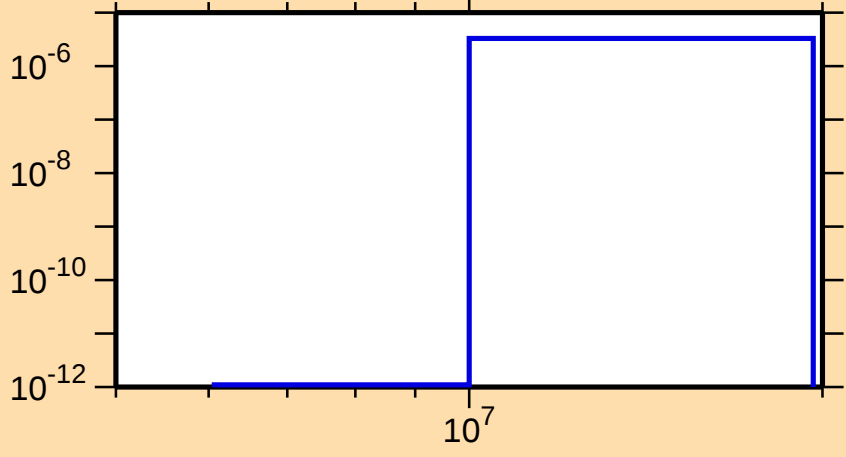
\sigma vs. E for ^{123}\text{Cs}(n,\text{He}3)
