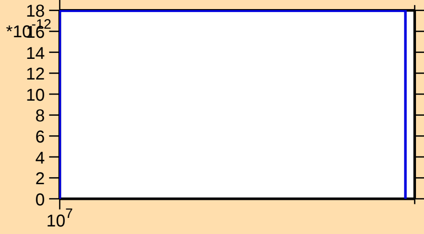
\sigma vs. E for ^{123}\text{Cs}(n,2n\alpha)
