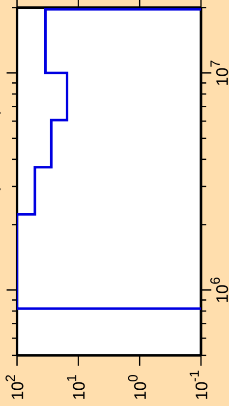
\Delta\sigma/\sigma vs. E for ^{123}\text{Cs}(n,n_{\text{cont}})
