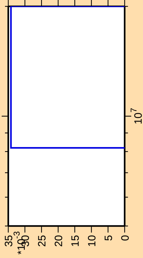
\Delta\sigma/\sigma vs. E for ^{123}\text{Cs}(\text{mt } 34)
