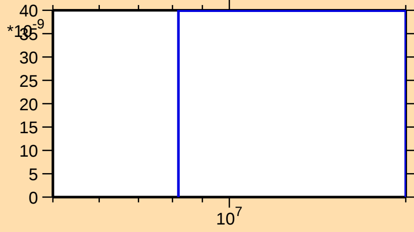
\sigma vs. E for ^{123}\text{Cs}(\text{mt } 45)
