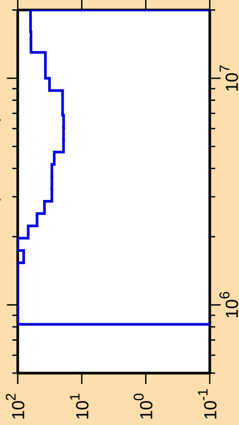
\Delta\sigma/\sigma vs. E for ^{125}\text{Cs}(n,\text{ncont.})
