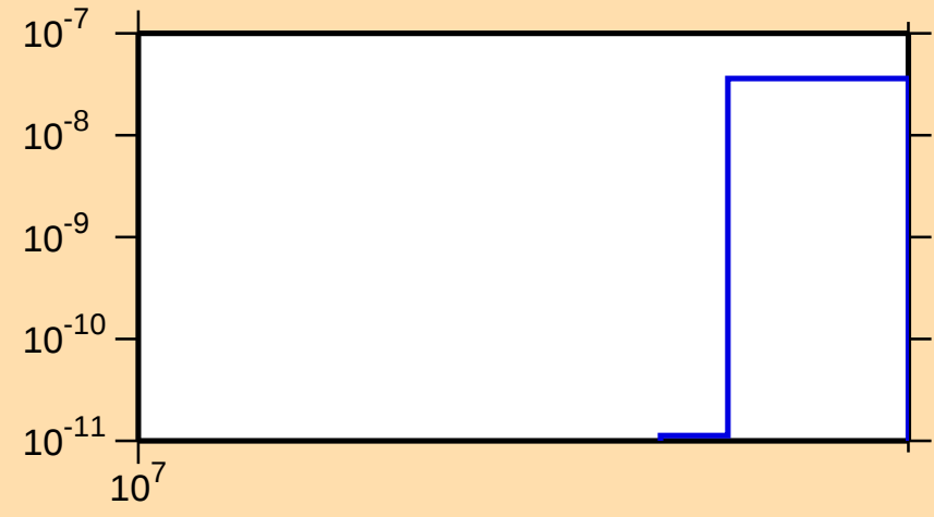
\sigma vs. E for ^{125}\text{Cs}(n,nt)
