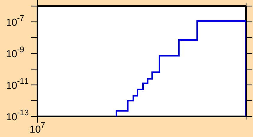
\sigma vs. E for ^{125}\text{Cs} (mt 45)
