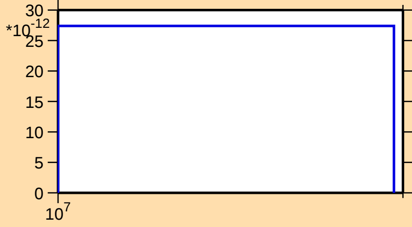
\sigma vs. E for ^{125}\text{Cs}(n,2n\alpha)
