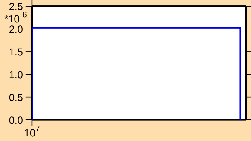
\sigma vs. E for ^{125}\text{Cs}(n,2np)
