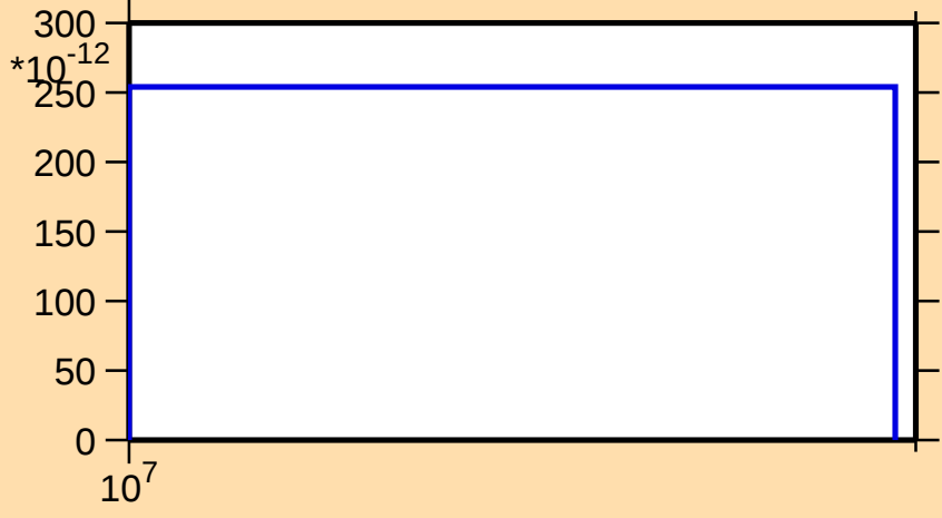
\sigma vs. E for ^{125}\text{Cs}(n,\text{nt})
