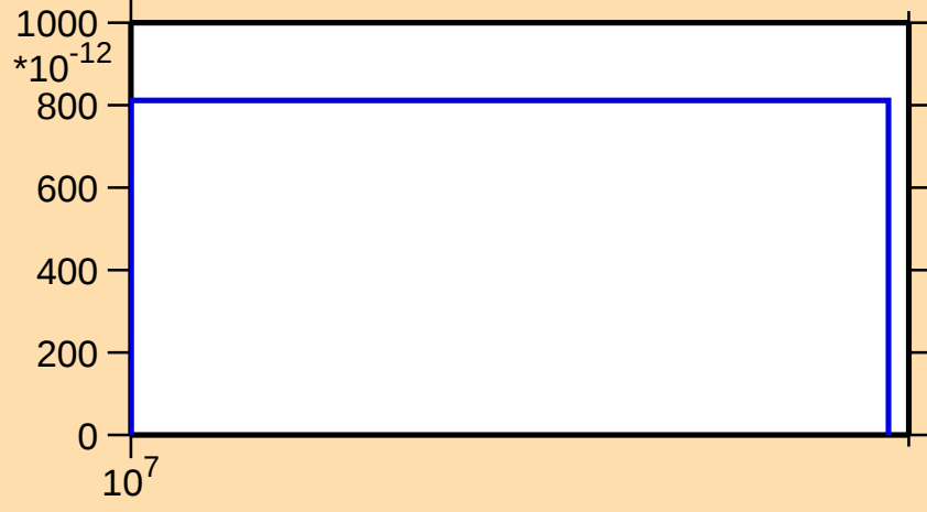
\sigma vs. E for ^{125}\text{Cs}(n,\text{pd})
