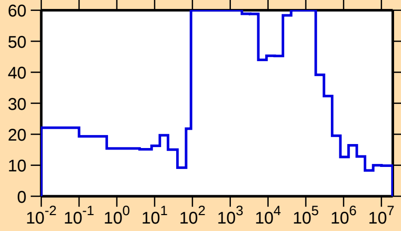
\Delta\sigma/\sigma vs. E for ^{125}\text{Cs}(n,\text{tot.})
