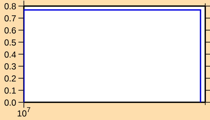
\sigma vs. E for ^{125}\text{Cs}(n,2n)
