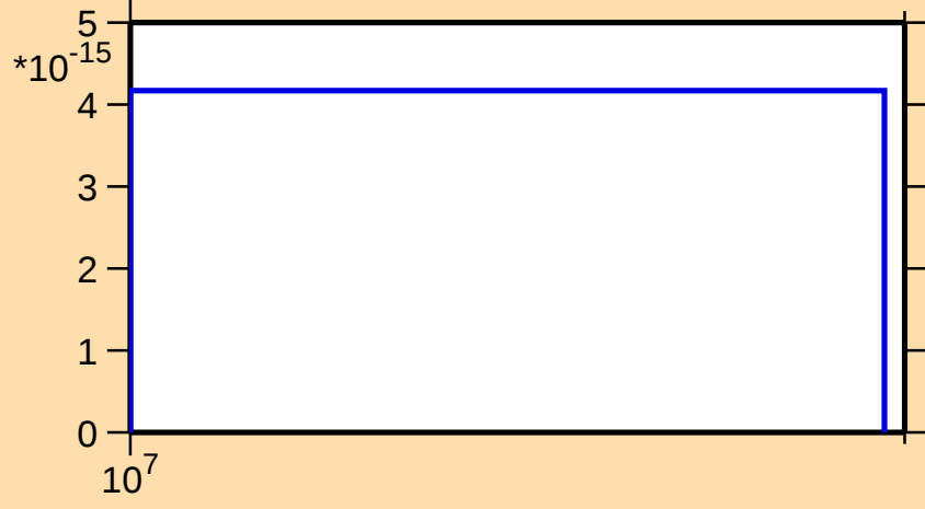
\sigma vs. E for ^{125}\text{Cs}(n,\text{pt})
