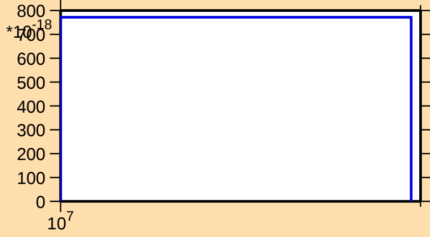
\sigma vs. E for ^{125}\text{Cs}(\text{mt } 34)
