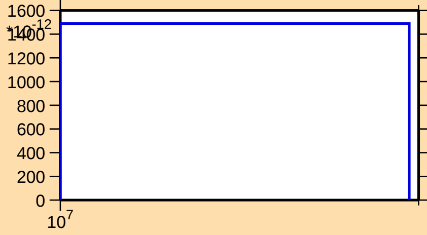
\sigma vs. E for ^{125}\text{Cs}(\text{mt } 45)
