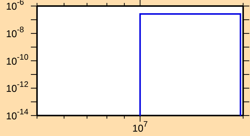
\sigma vs. E for ^{125}\text{Cs}(n,\text{He3})
