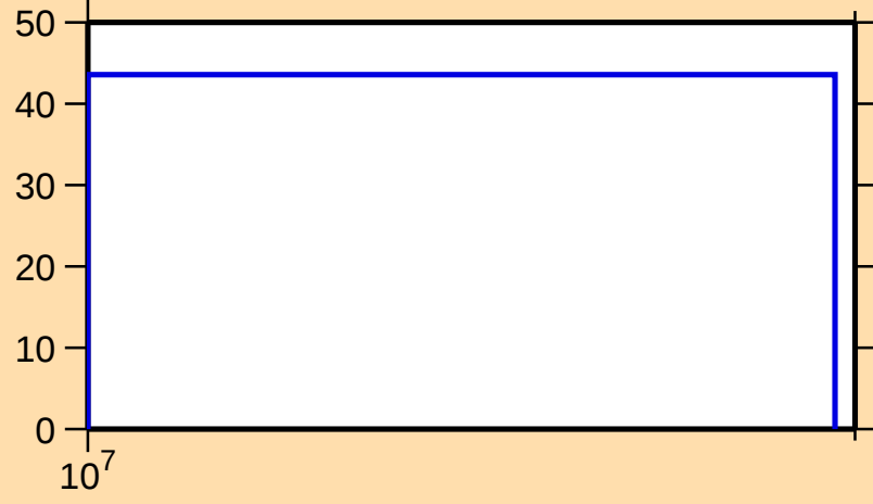
\Delta\sigma/\sigma vs. E for ^{125}\text{Cs}(n,\text{inel.})
