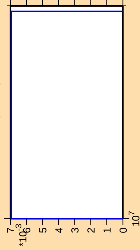
\Delta\sigma/\sigma vs. E for ^{125}\text{Cs}(\text{mt } 34)
