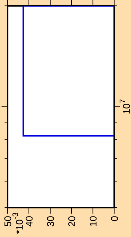
\Delta\sigma/\sigma vs. E for ^{125}\text{Cs}(n,\text{pt})
