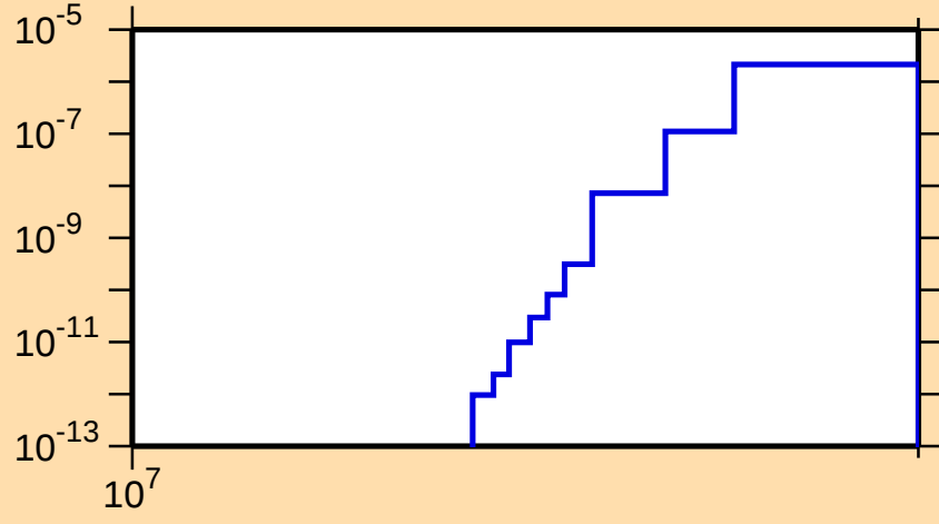
\sigma vs. E for ^{126}\text{Cs}(n,2n\alpha)
