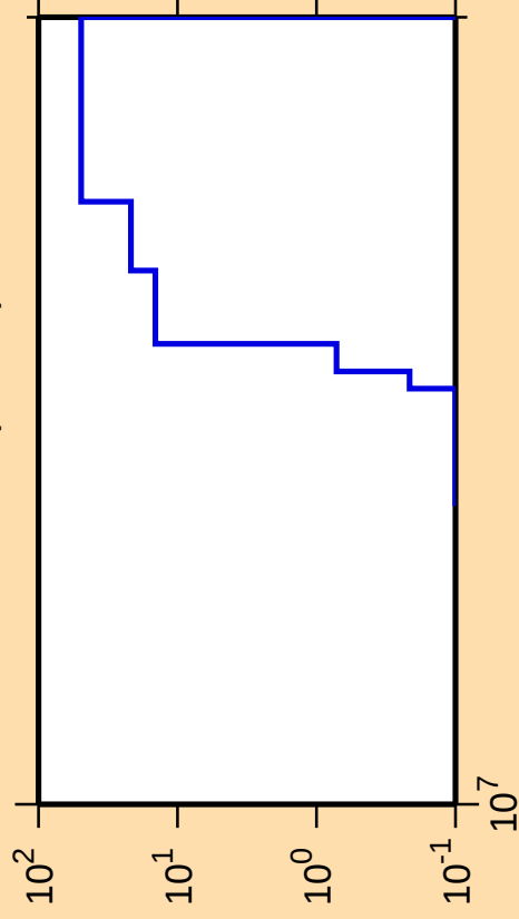
\Delta\sigma/\sigma vs. E for ^{126}\text{Cs}(\text{mt } 45)
