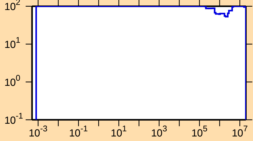
\Delta\sigma/\sigma vs. E for ^{126}\text{Cs}(n,p)
