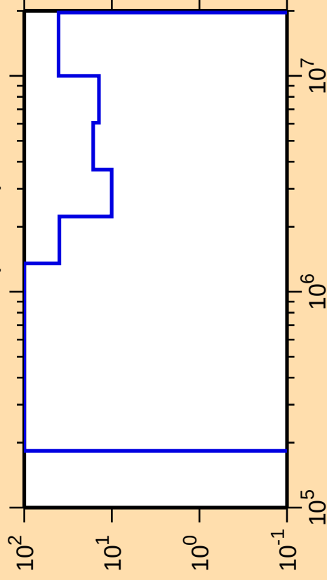
\Delta\sigma/\sigma vs. E for ^{126}\text{Cs}(n,\text{inel.})
