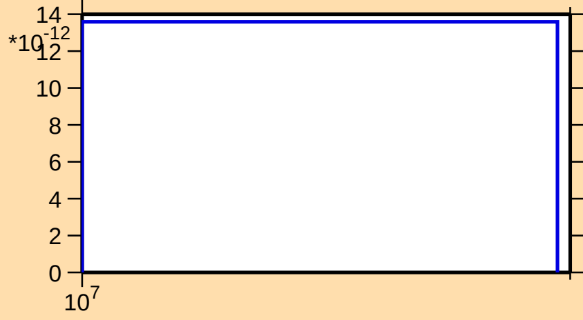
\sigma vs. E for ^{126}\text{Cs}(\text{mt } 45)
