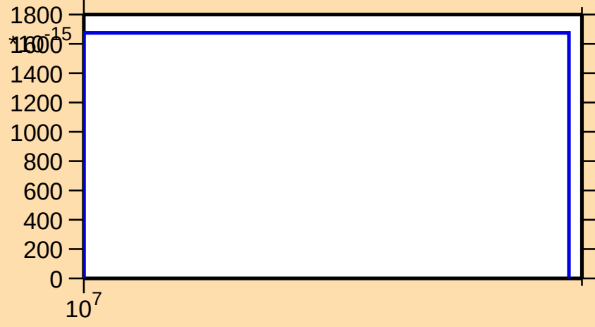
\sigma vs. E for ^{126}\text{Cs}(\text{mt117})
