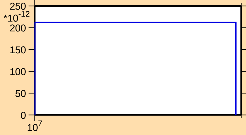
\sigma vs. E for ^{126}\text{Cs}(n,nt)
