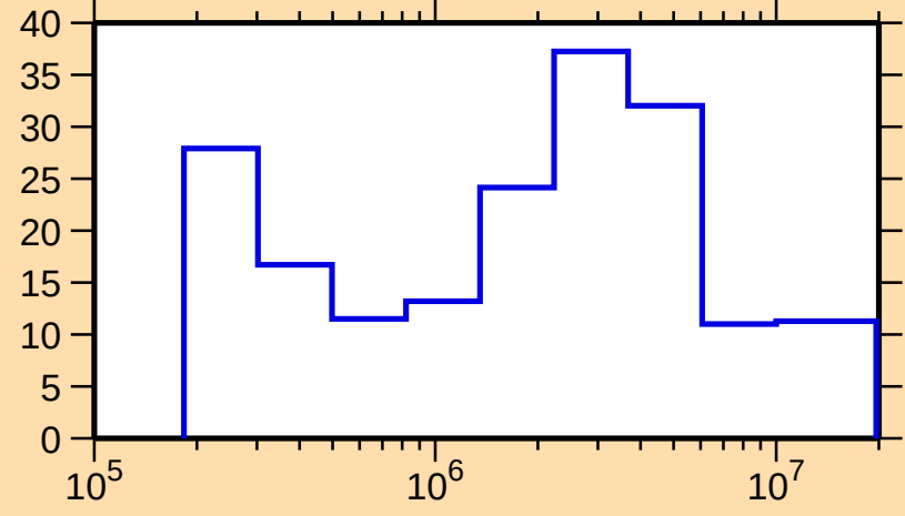
\Delta\sigma/\sigma vs. E for ^{126}\text{Cs}(n,\text{el.})
