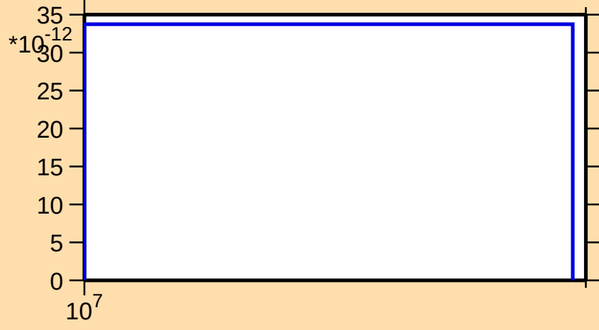
\sigma vs. E for ^{126}\text{Cs}(n,\text{pd})
