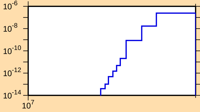
\sigma vs. E for ^{132}\text{Cs}(n,2n\alpha)
