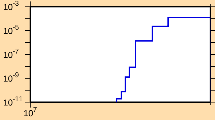
\sigma vs. E for ^{132}\text{Cs}(n,2np)
