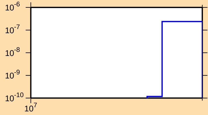
\sigma vs. E for ^{132}\text{Cs}(n,nt)
