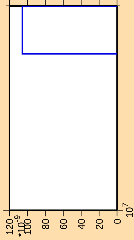
\Delta\sigma/\sigma vs. E for ^{132}\text{Cs} (mt 11)
