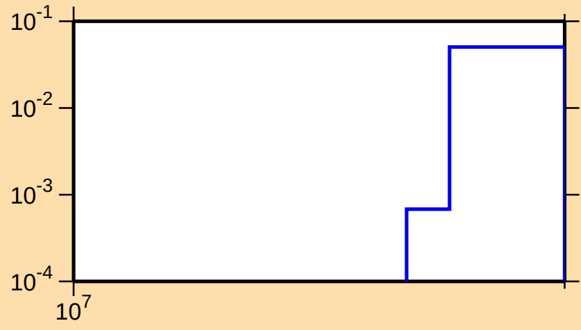
\sigma vs. E for ^{132}\text{Cs}(n,3n)
