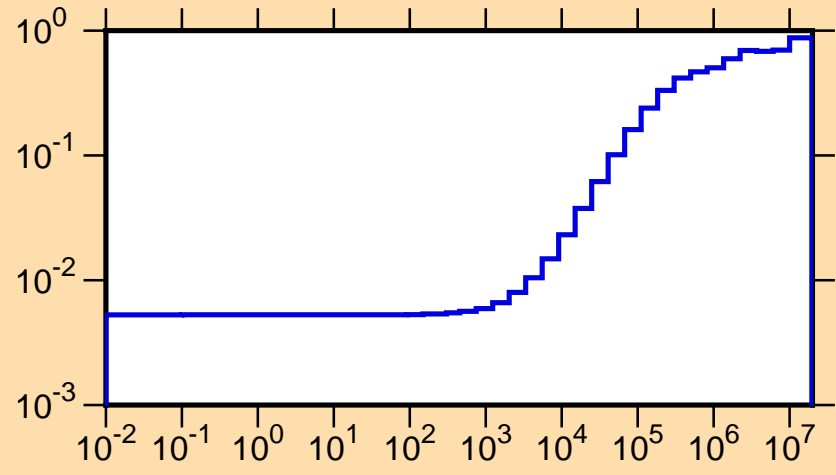
\mu vs. E for ^{132}\text{Cs}(\text{mt251})
