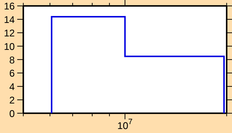
\Delta\sigma/\sigma vs. E for ^{132}\text{Cs}(n,2n)
