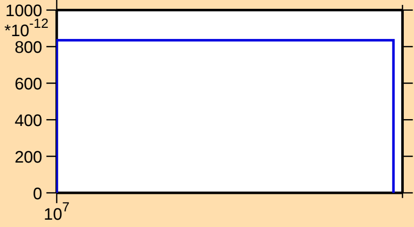
\sigma vs. E for ^{132}\text{Cs}(n,\text{He}3)
