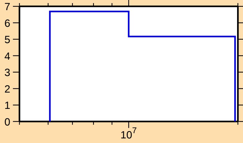
\Delta\sigma/\sigma vs. E for ^{132}\text{Cs}(n,\text{nonel.})
