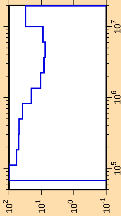
\Delta\sigma/\sigma vs. E for ^{132}\text{Cs}(n,\text{inel.})
