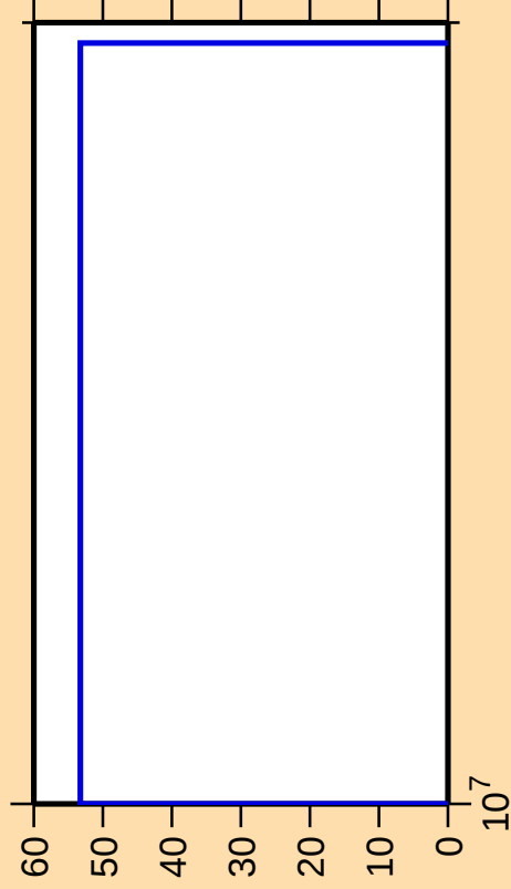
\Delta\sigma/\sigma vs. E for ^{132}\text{Cs}(n,3n)
