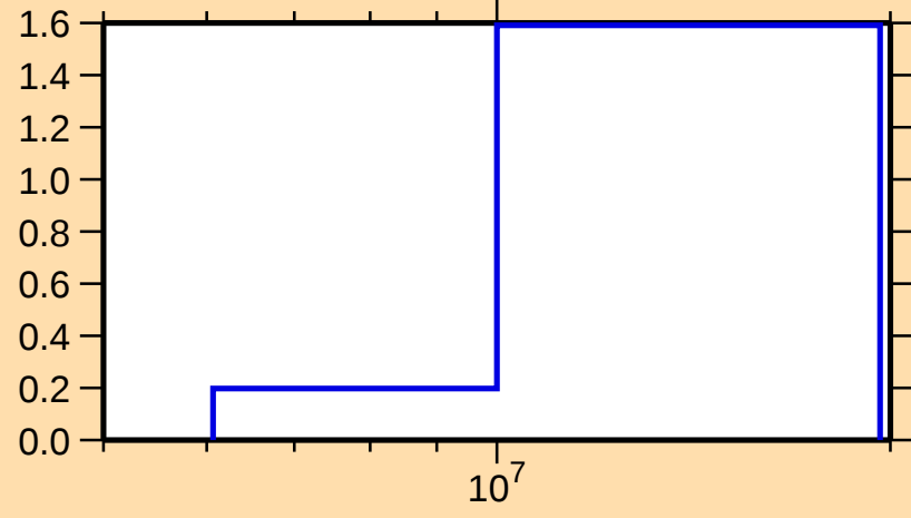
\sigma vs. E for ^{132}\text{Cs}(n,2n)
