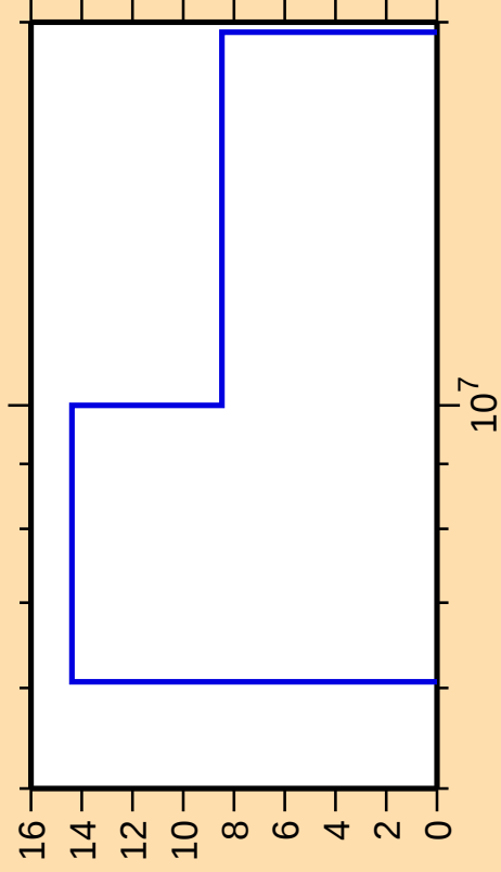
\Delta\sigma/\sigma vs. E for ^{132}\text{Cs}(n,2n)
