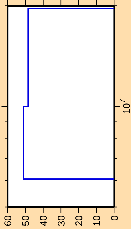
\Delta\sigma/\sigma vs. E for ^{132}\text{Cs}(n,n_1)
