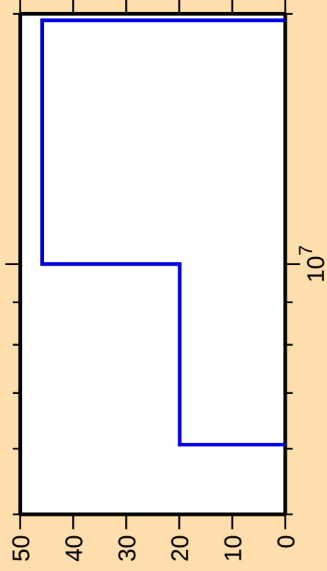
\Delta\sigma/\sigma vs. E for ^{132}\text{Cs}(n,n\text{cont.})
