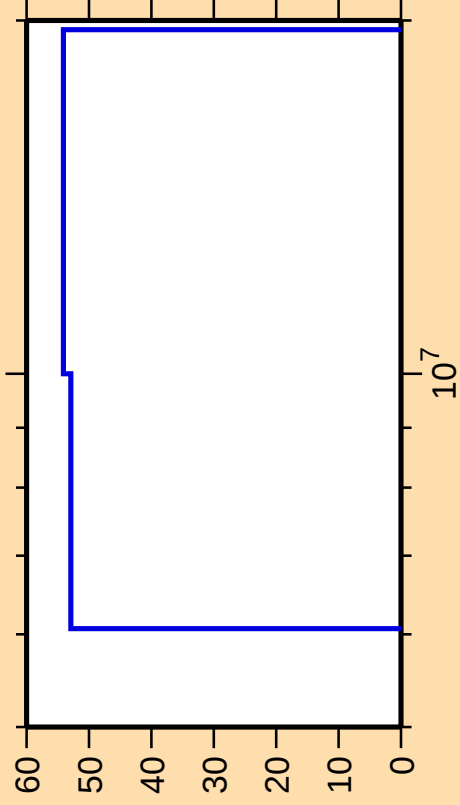
\Delta\sigma/\sigma vs. E for ^{132}\text{Cs}(n,p)
