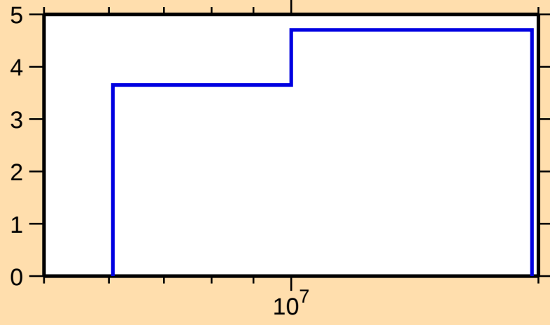
\Delta\sigma/\sigma vs. E for ^{132}\text{Cs}(n,\text{tot.})
