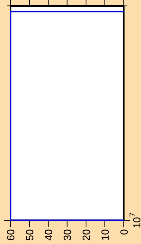
\Delta\sigma/\sigma vs. E for ^{132}\text{Cs}(n,\text{nt})
