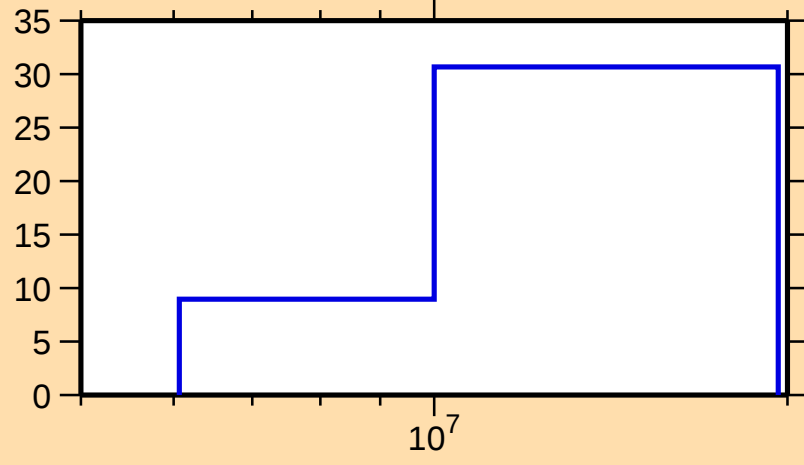
\Delta\sigma/\sigma vs. E for ^{132}\text{Cs}(n,\text{inel.})
