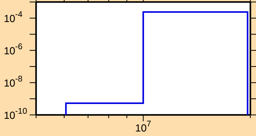
\sigma vs. E for ^{132}\text{Cs}(n,n\alpha)
