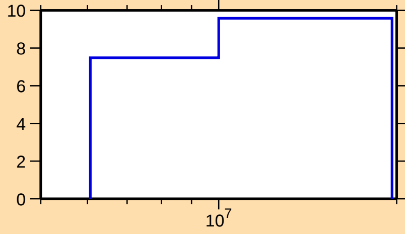
\Delta\sigma/\sigma vs. E for ^{132}\text{Cs}(n,\text{el.})
