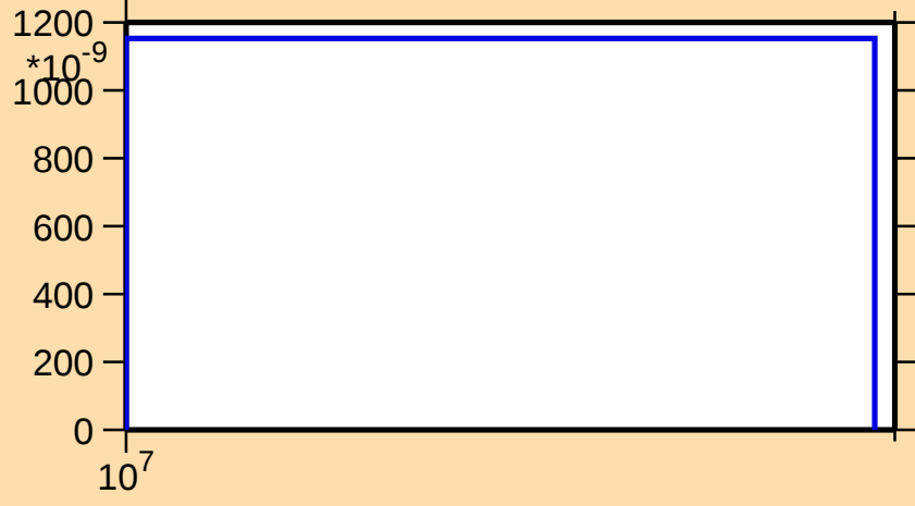
\sigma vs. E for ^{132}\text{Cs}(n,\text{nd})
