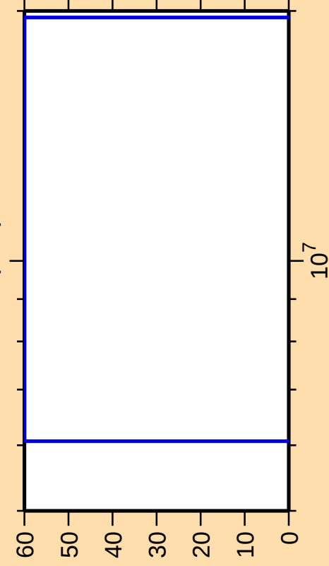
\Delta\sigma/\sigma vs. E for ^{132}\text{Cs}(n,\alpha)
