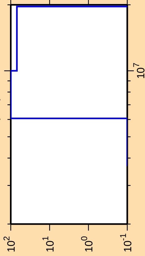
\Delta\sigma/\sigma vs. E for ^{132}\text{Cs}(n,d)
