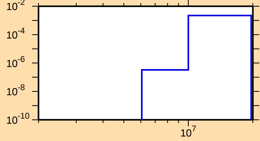
\sigma vs. E for ^{132}\text{Cs}(n,d)
