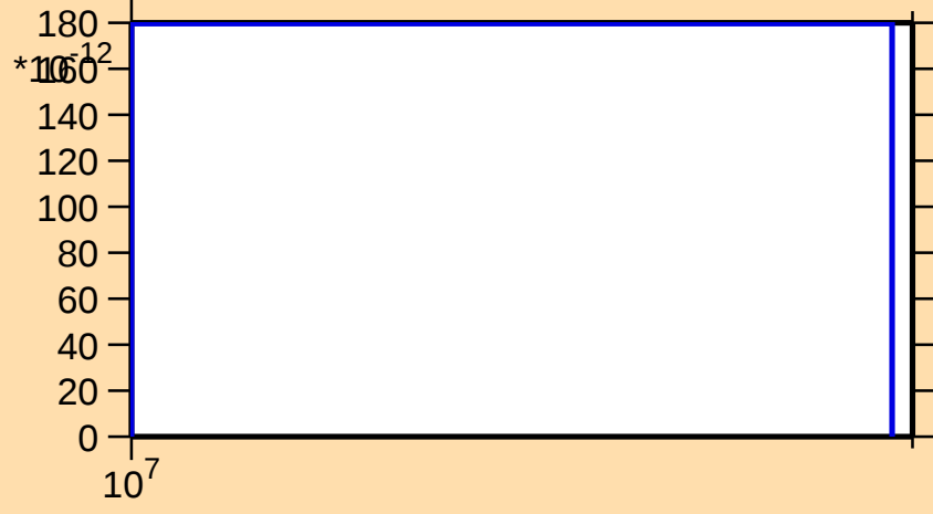
\sigma vs. E for ^{132}\text{Cs}(n,p\alpha)
