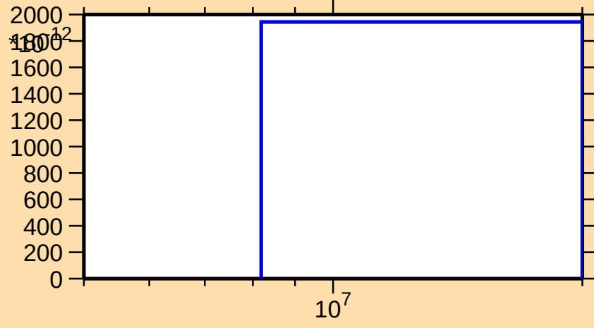
\sigma vs. E for ^{132}\text{Cs}(n,\text{nt})
