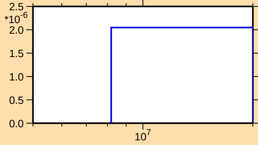
\sigma vs. E for ^{132}\text{Cs}(n,2np)
