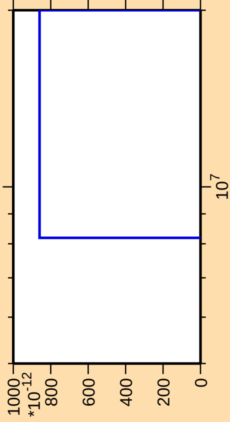
\Delta\sigma/\sigma vs. E for ^{132}\text{Cs}(\text{mt 11})
