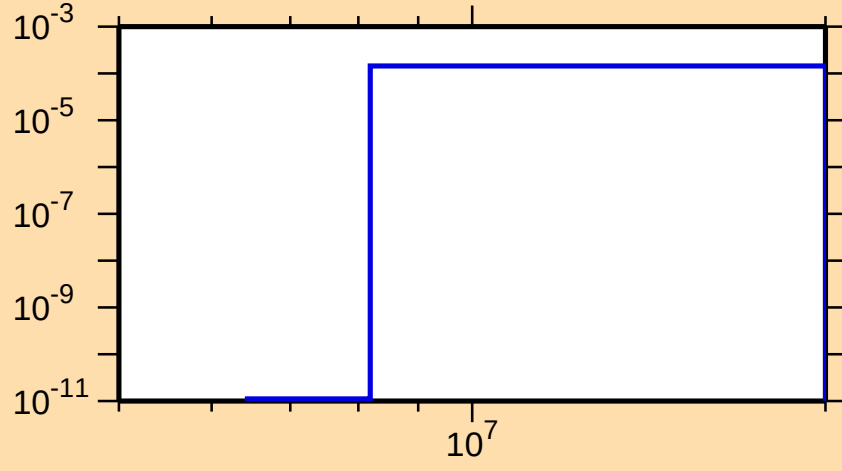
\sigma vs. E for ^{132}\text{Cs}(n,t)
