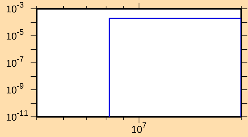
\sigma vs. E for ^{132}\text{Cs}(n,n\alpha)
