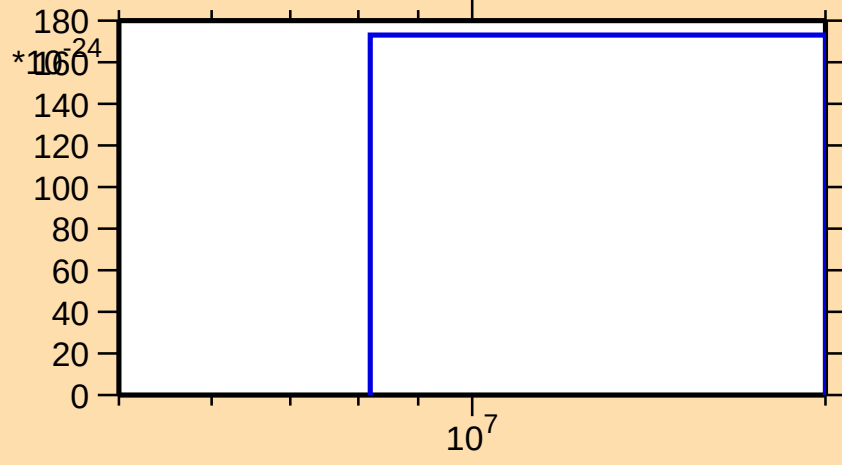
\sigma vs. E for ^{132}\text{Cs}(\text{mt 11})
