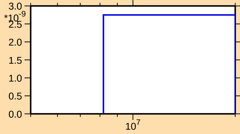
\sigma vs. E for ^{132}\text{Cs}(n,2n\alpha)
