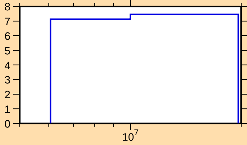
\Delta\sigma/\sigma vs. E for ^{134}\text{Cs}(n,\text{el.})
