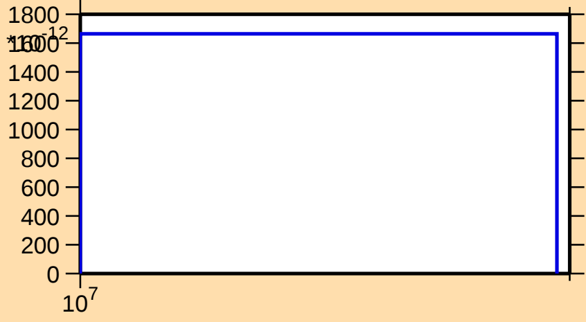
\sigma vs. E for ^{134}\text{Cs}(n,\text{nt})
