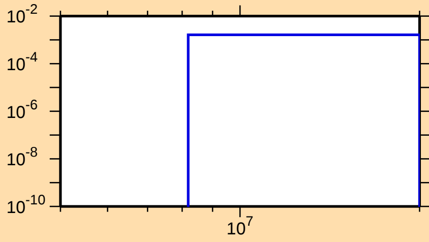
\sigma vs. E for ^{134}\text{Cs}(n,np)
