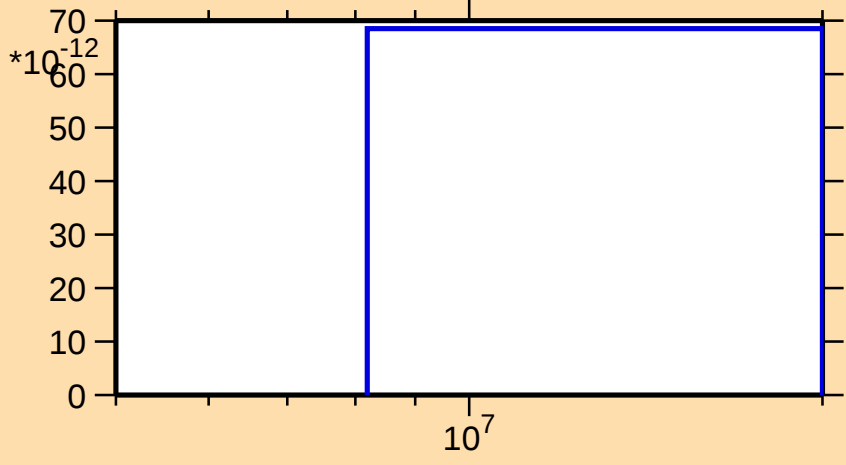
\sigma vs. E for ^{134}\text{Cs}(n,\text{He}3)
