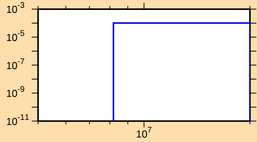
\sigma vs. E for ^{134}\text{Cs}(n,n\alpha)
