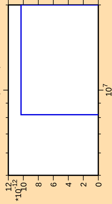
\Delta\sigma/\sigma vs. E for ^{134}\text{Cs}(\text{mt 11})
