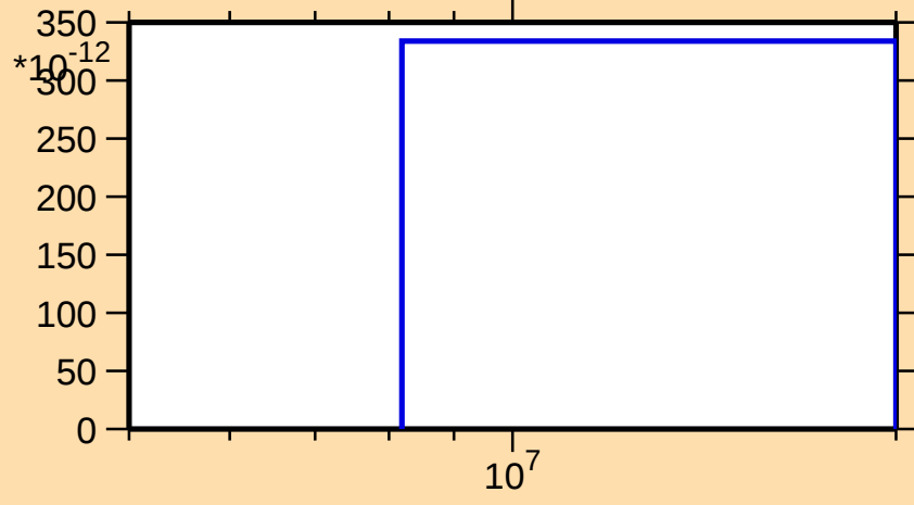
\sigma vs. E for ^{134}\text{Cs}(n,2n\alpha)
