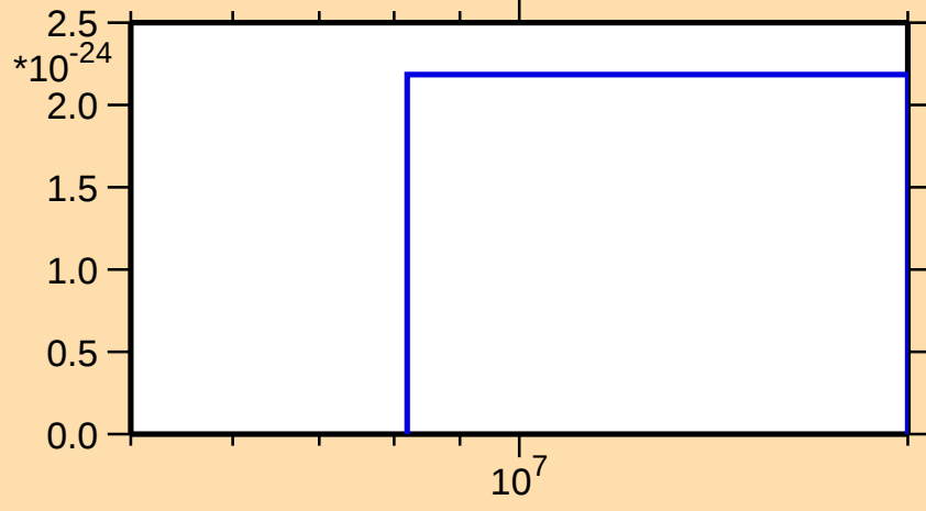
\sigma vs. E for ^{134}\text{Cs}(\text{mt 11})
