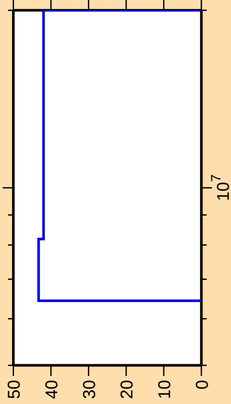
\Delta\sigma/\sigma vs. E for ^{134}\text{Cs}(n,p)
