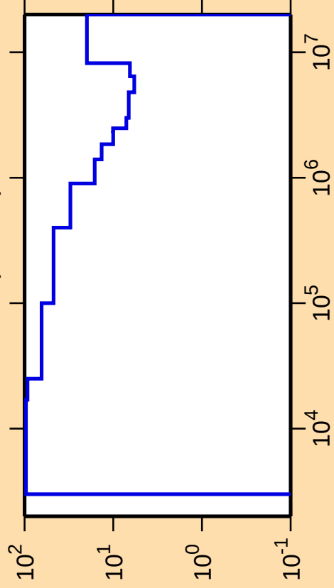
\Delta\sigma/\sigma vs. E for ^{134}\text{Cs}(n,\text{inel.})
