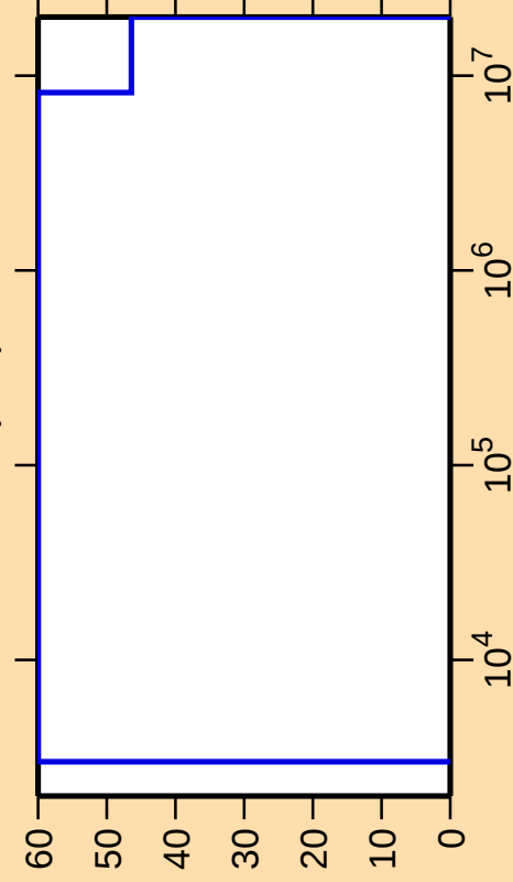
\Delta\sigma/\sigma vs. E for ^{134}\text{Cs}(n,\alpha)
