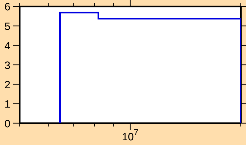
\Delta\sigma/\sigma vs. E for ^{134}\text{Cs}(n,\text{nonel.})
