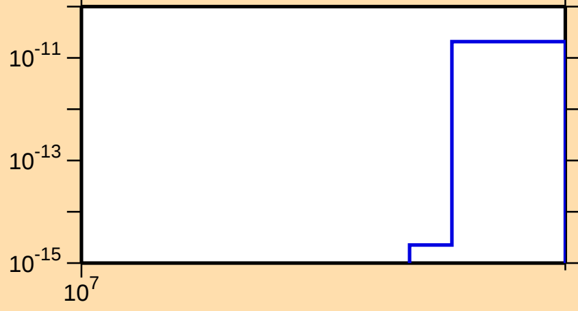
\sigma vs. E for ^{137}\text{Cs}(n,2n\alpha)
