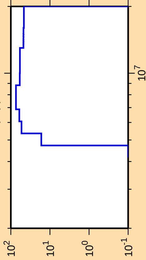
\Delta\sigma/\sigma vs. E for ^{137}\text{Cs}(n,p)
