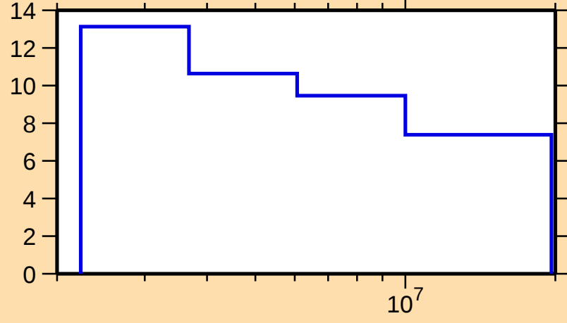
\Delta\sigma/\sigma vs. E for ^{137}\text{Cs}(n,n\text{onel.})
