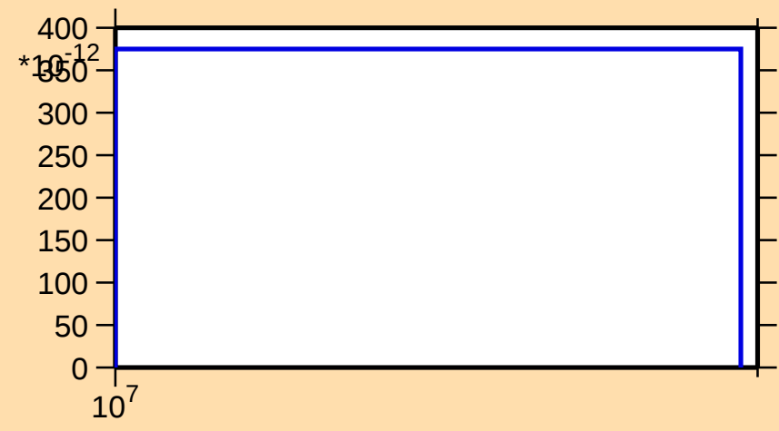
\sigma vs. E for ^{137}\text{Cs}(n,\text{nt})
