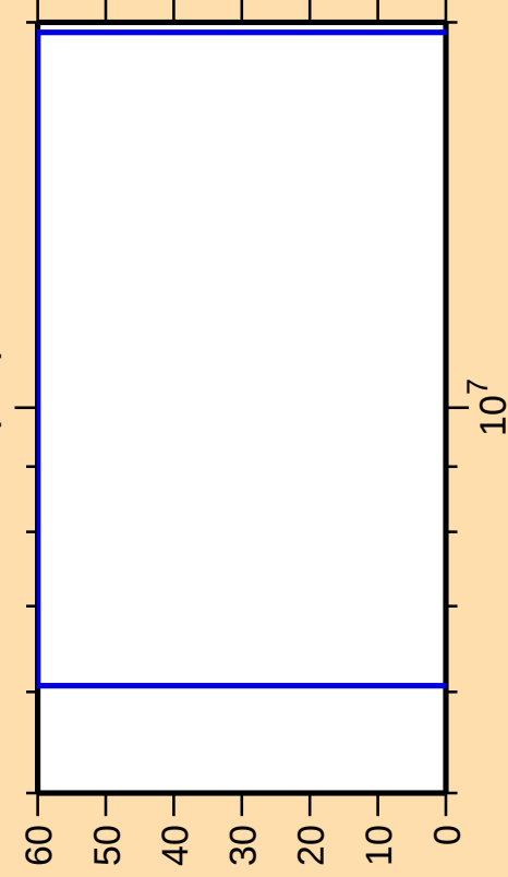
\Delta\sigma/\sigma vs. E for ^{137}\text{Cs}(n,d)
