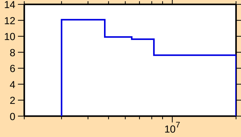
\Delta\sigma/\sigma vs. E for ^{137}\text{Cs}(n,n\text{nonel.})
