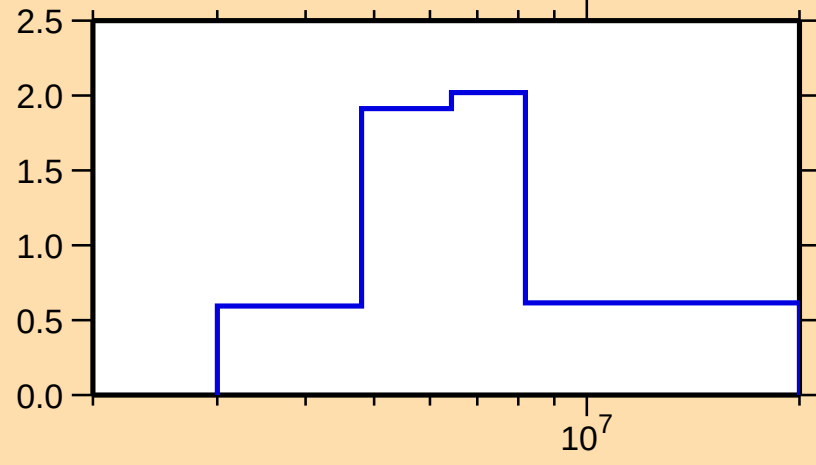
\sigma vs. E for ^{137}\text{Cs}(n,n\text{cont.})
