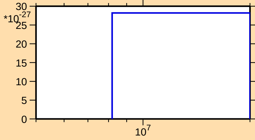
\sigma vs. E for ^{137}\text{Cs} (mt 11)
