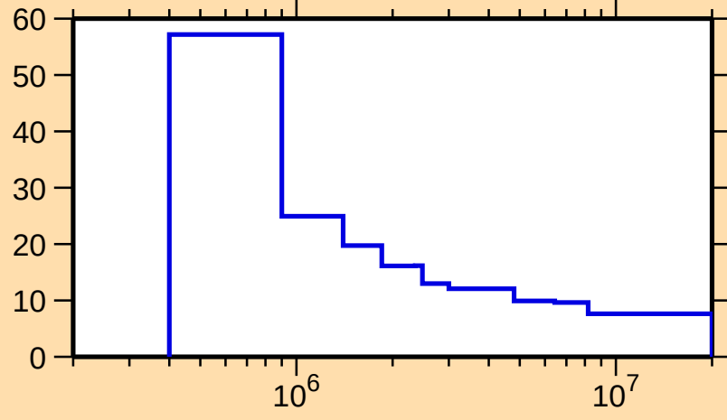
\Delta\sigma/\sigma vs. E for ^{137}\text{Cs}(n,\text{nonel.})
