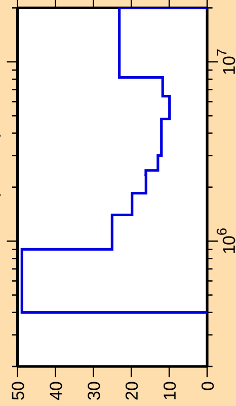
\Delta\sigma/\sigma vs. E for ^{137}\text{Cs}(n,\text{inel.})
