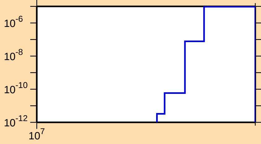
\sigma vs. E for ^{70}\text{Cu}(n,2np)
