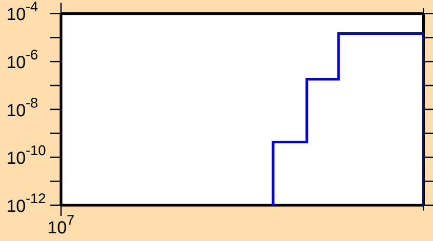
\sigma vs. E for ^{70}\text{Cu}(n,nt)
