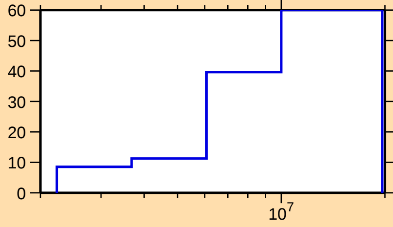
\Delta\sigma/\sigma vs. E for ^{70}\text{Cu}(n,ncont.)
