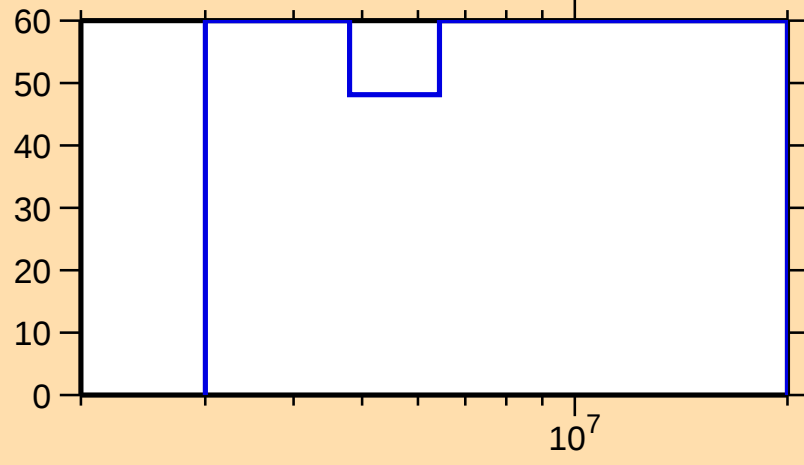
\Delta\sigma/\sigma vs. E for ^{70}\text{Cu}(n,\gamma)
