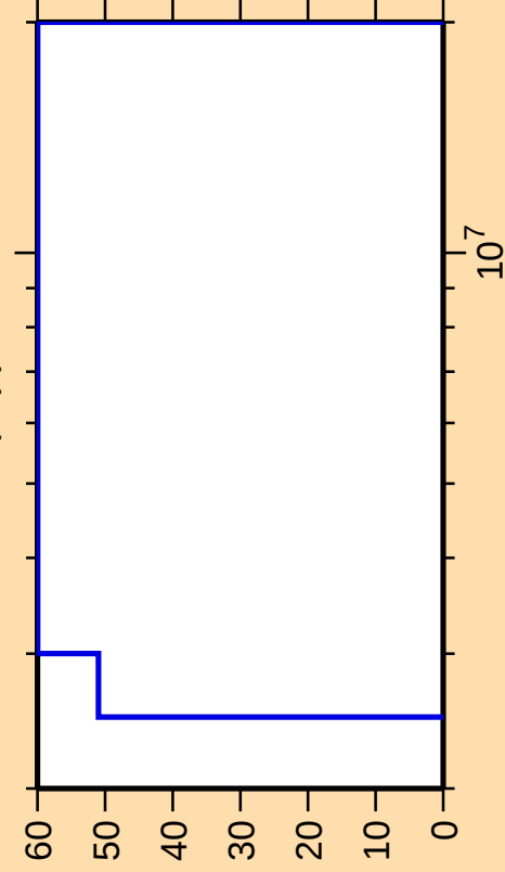
\Delta\sigma/\sigma vs. E for ^{70}\text{Cu}(n,p)
