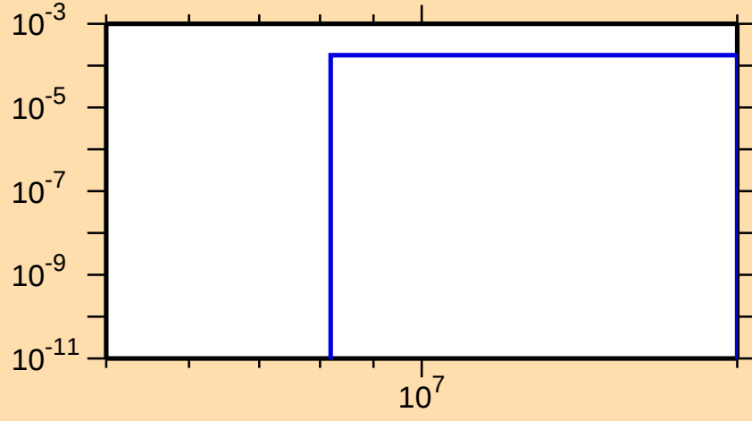
\sigma vs. E for ^{70}\text{Cu}(n,d)
