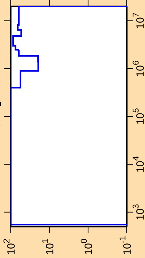
\Delta\sigma/\sigma vs. E for ^{70}\text{Cu}(n,n_1)
