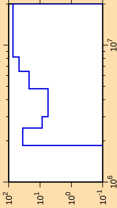
\Delta\sigma/\sigma vs. E for ^{70}\text{Cu}(n,n\text{cont.})
