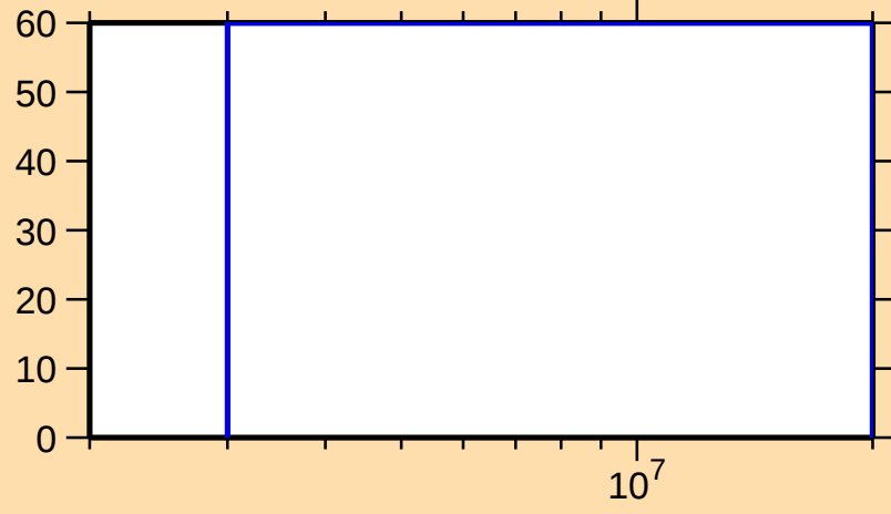
\Delta\sigma/\sigma vs. E for ^{70}\text{Cu}(n,p)
