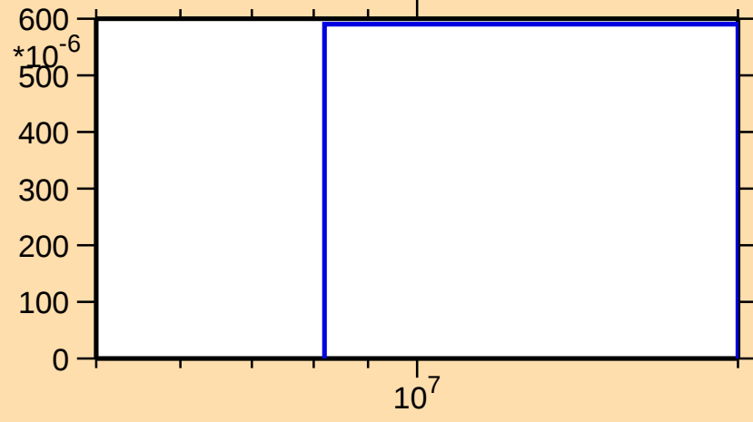
\sigma vs. E for ^{70}\text{Cu}(n,np)
