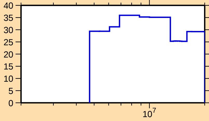
\Delta\sigma/\sigma vs. E for ^{72}\text{Cu}(n,\text{nonel.})
