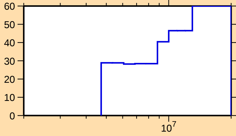
\Delta\sigma/\sigma vs. E for ^{72}\text{Cu}(n,\text{el.})
