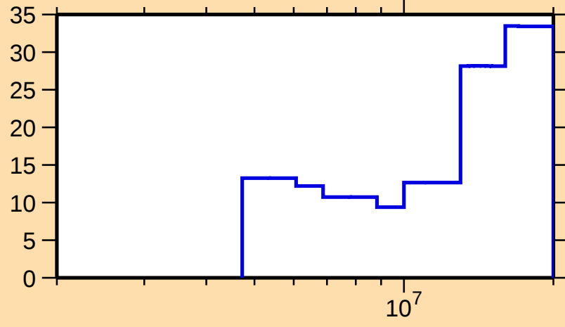
\Delta\sigma/\sigma vs. E for ^{72}\text{Cu}(n,\text{tot.})
