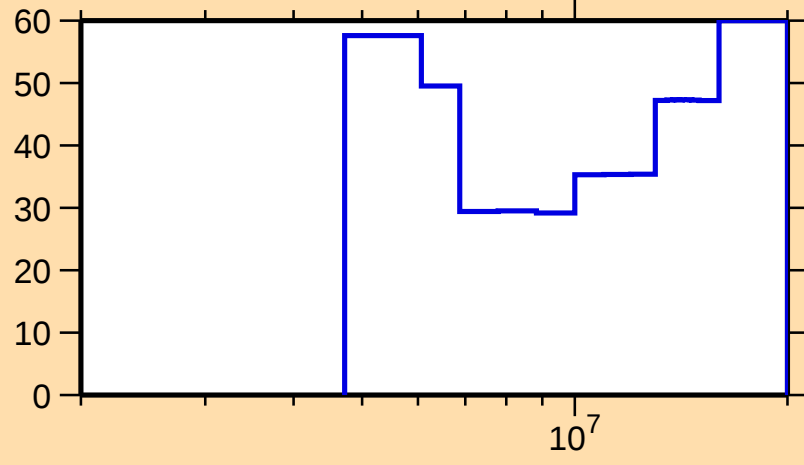
\Delta\sigma/\sigma vs. E for ^{72}\text{Cu}(n,n\text{cont.})
