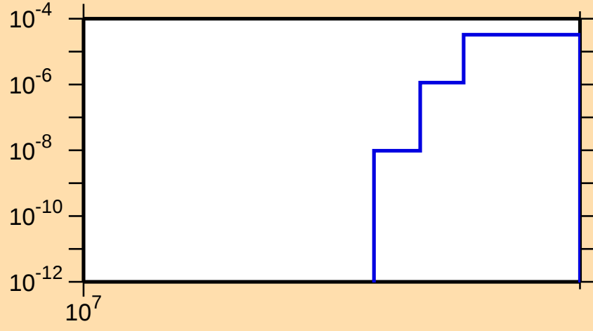
\sigma vs. E for ^{72}\text{Cu}(n,\text{nd})
