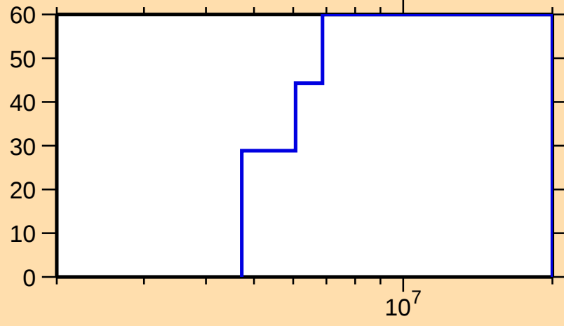
\Delta\sigma/\sigma vs. E for ^{72}\text{Cu}(n,\text{inel.})
