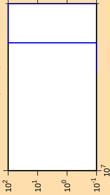
\Delta\sigma/\sigma vs. E for ^{72}\text{Cu}(n,2n\alpha)
