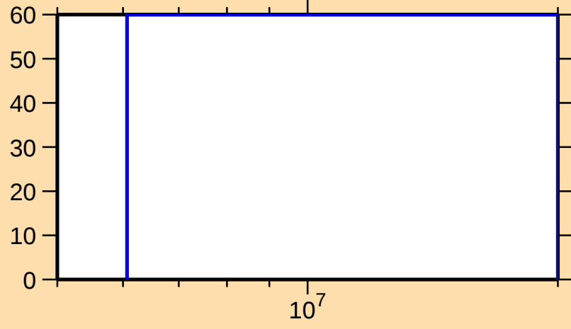
\Delta\sigma/\sigma vs. E for ^{72}\text{Cu}(n,\gamma)
