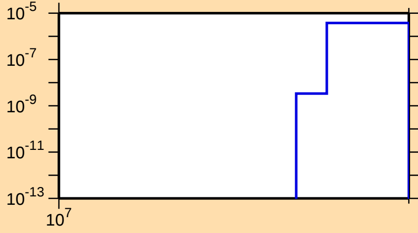
\sigma vs. E for ^{72}\text{Cu}(n,nt)
