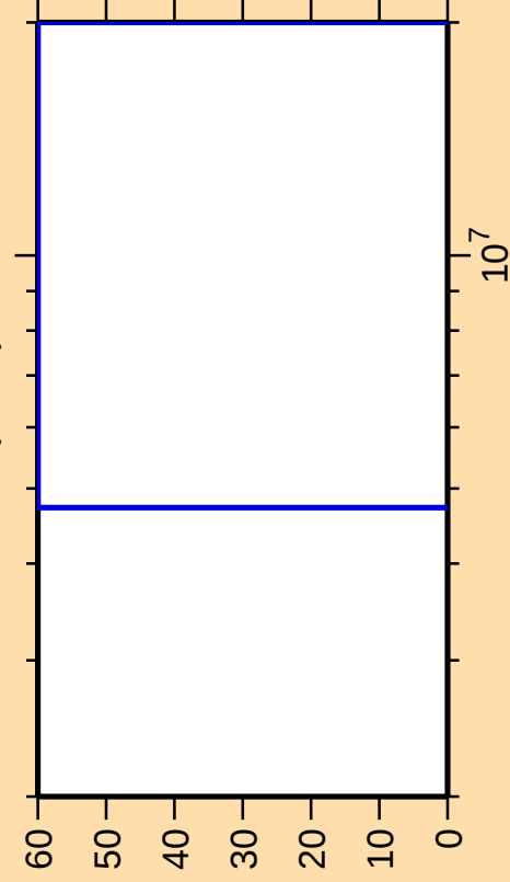
\Delta\sigma/\sigma vs. E for ^{72}\text{Cu}(n,2n)
