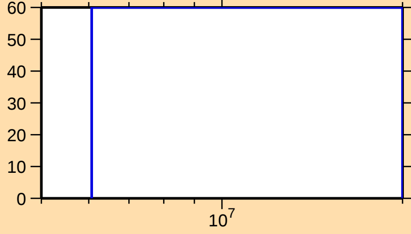
\Delta\sigma/\sigma vs. E for ^{72}\text{Cu}(n,p)
