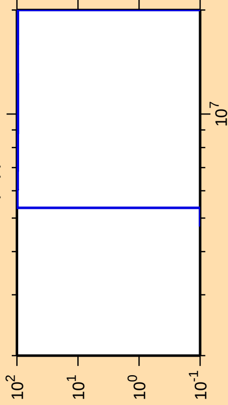
\Delta\sigma/\sigma vs. E for ^{72}\text{Cu}(n,p)
