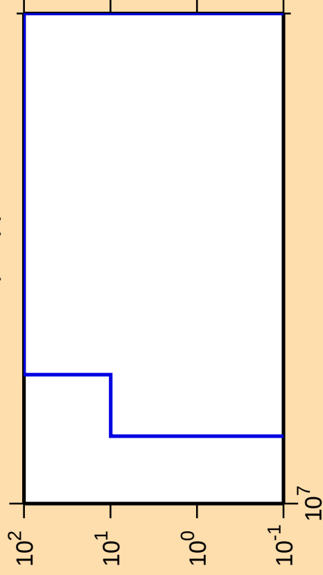
\Delta\sigma/\sigma vs. E for ^{72}\text{Cu}(n,np)
