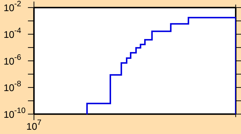
\sigma vs. E for ^{72}\text{Cu}(n,np)
