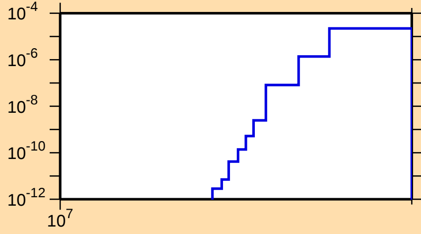
\sigma vs. E for ^{72}\text{Cu}(n,n\alpha)
