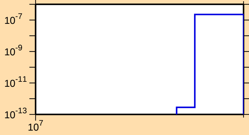
\sigma vs. E for ^{72}\text{Cu}(n,2np)
