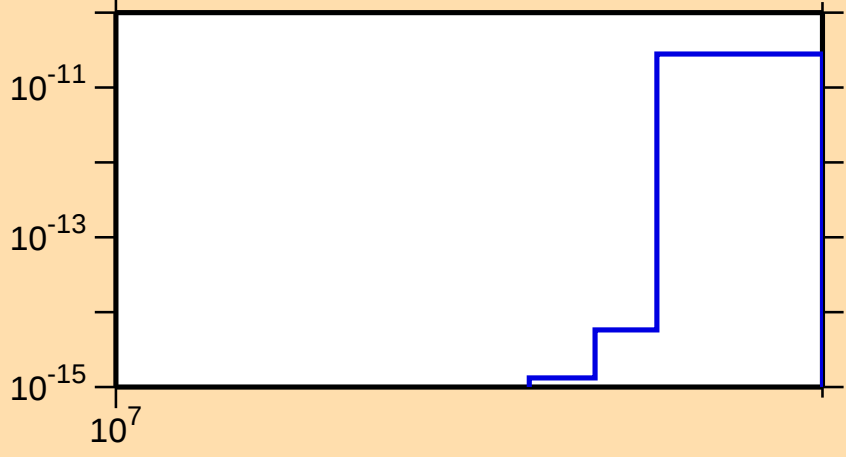
\sigma vs. E for ^{72}\text{Cu}(n,2n\alpha)
