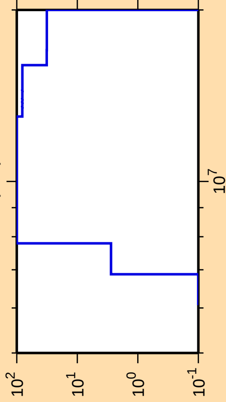
\Delta\sigma/\sigma vs. E for ^{72}\text{Cu}(n,\alpha)
