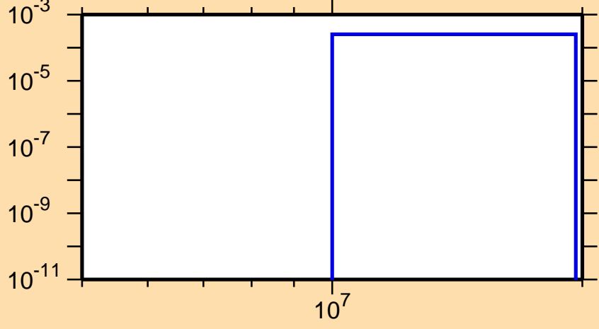
\sigma vs. E for ^{72}\text{Cu}(n,d)
