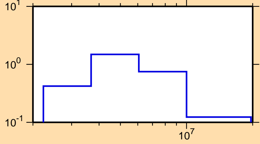
\sigma vs. E for ^{72}\text{Cu}(n,n\text{cont.})
