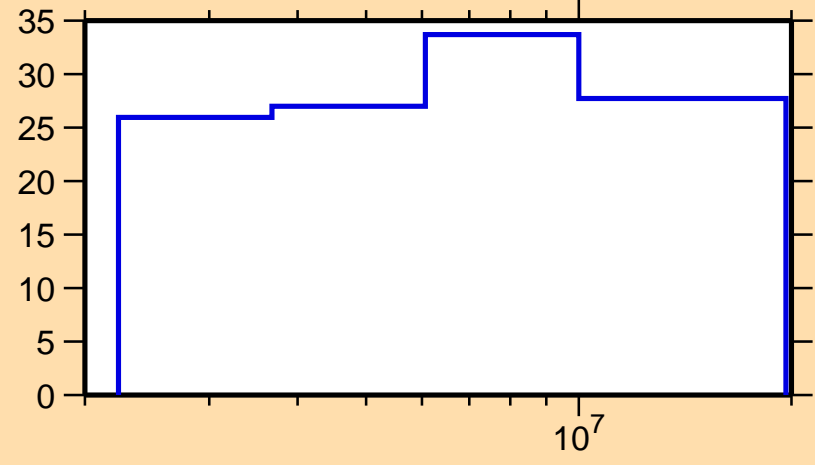
\Delta\sigma/\sigma vs. E for ^{72}\text{Cu}(n,n\text{onel.})
