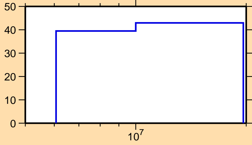
\Delta\sigma/\sigma vs. E for ^{72}\text{Cu}(n,ncont.)
