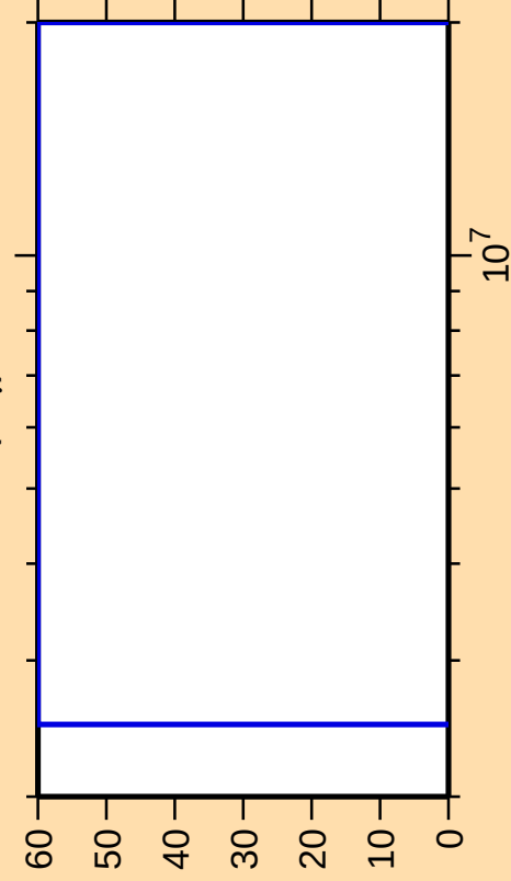
\Delta\sigma/\sigma vs. E for ^{72}\text{Cu}(n,\gamma)
