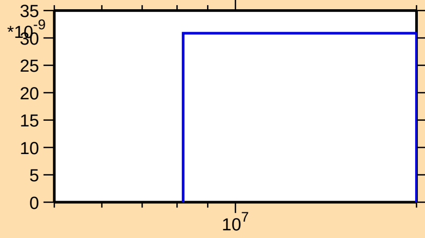
\sigma vs. E for ^{72}\text{Cu}(n,nt)
