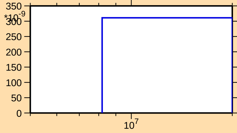
\sigma vs. E for ^{72}\text{Cu}(n,\text{nd})
