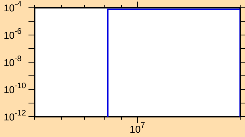
\sigma vs. E for ^{72}\text{Cu}(n,t)
