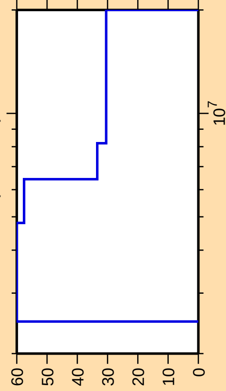
\Delta\sigma/\sigma vs. E for ^{72}\text{Cu}(n,n\text{cont.})
