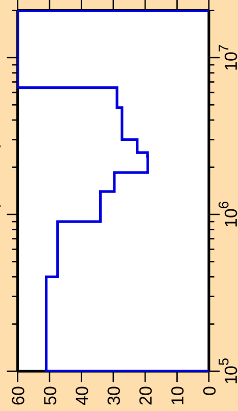
\Delta\sigma/\sigma vs. E for ^{72}\text{Cu}(n,\text{inel.})
