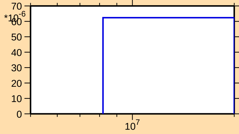
\sigma vs. E for ^{72}\text{Cu}(n,np)
