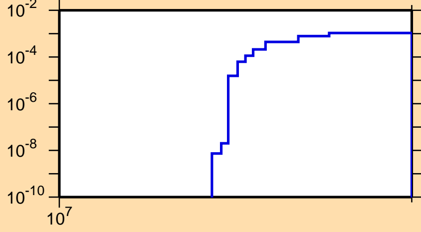
\sigma vs. E for ^{262}\alpha )
