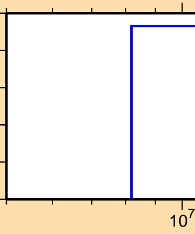
\sigma vs. E for ^{262}
