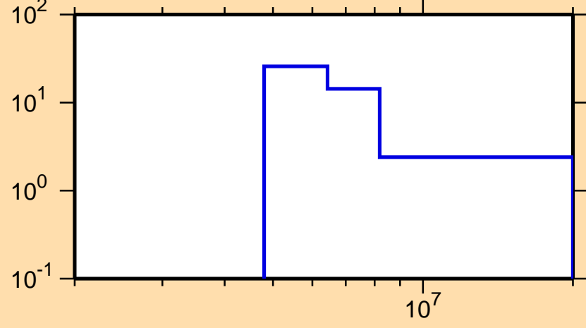
\Delta\sigma/\sigma vs. E for ^{262}
